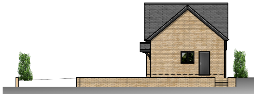
SECTIONAL VIEW 2 1:200
