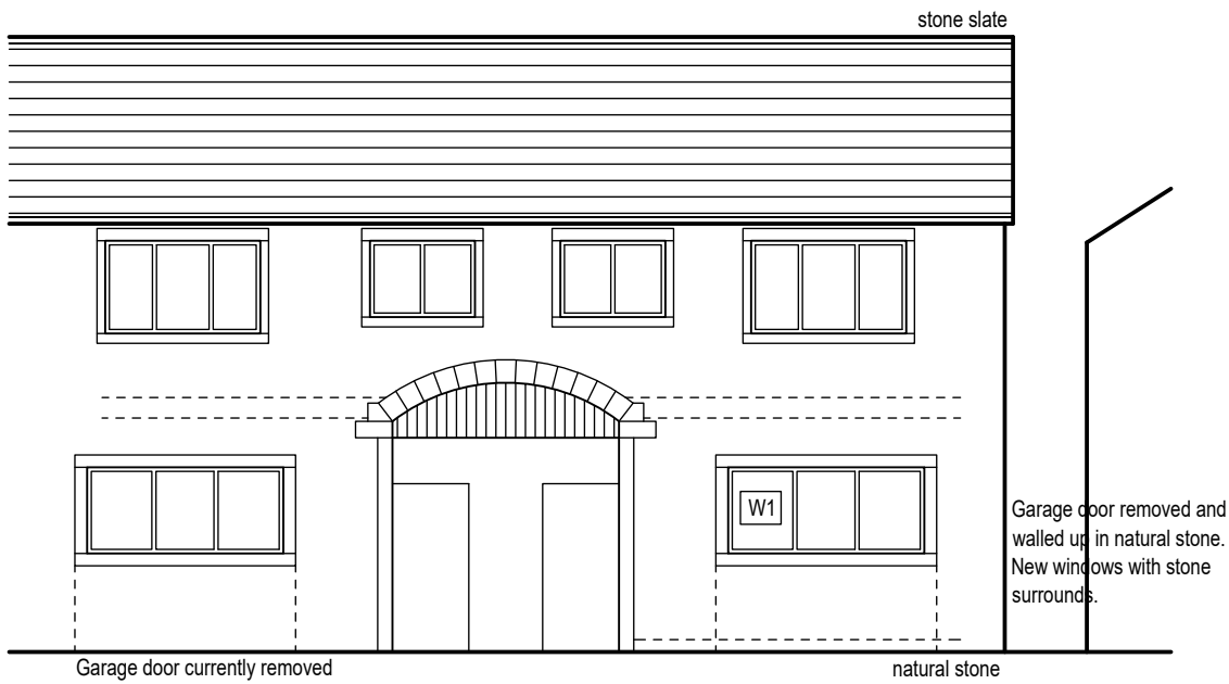
Proposed front/west facing elevation (1:100)
