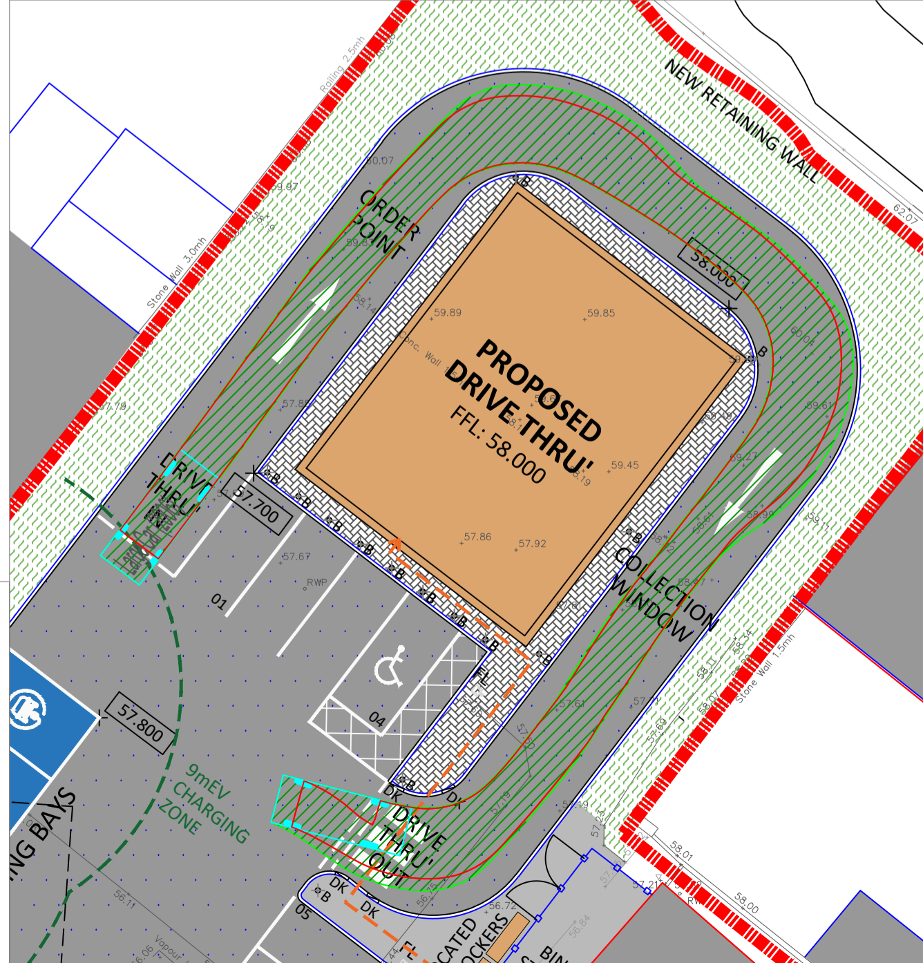
Swept Path Analysis - Large Car - Scale 1/200
