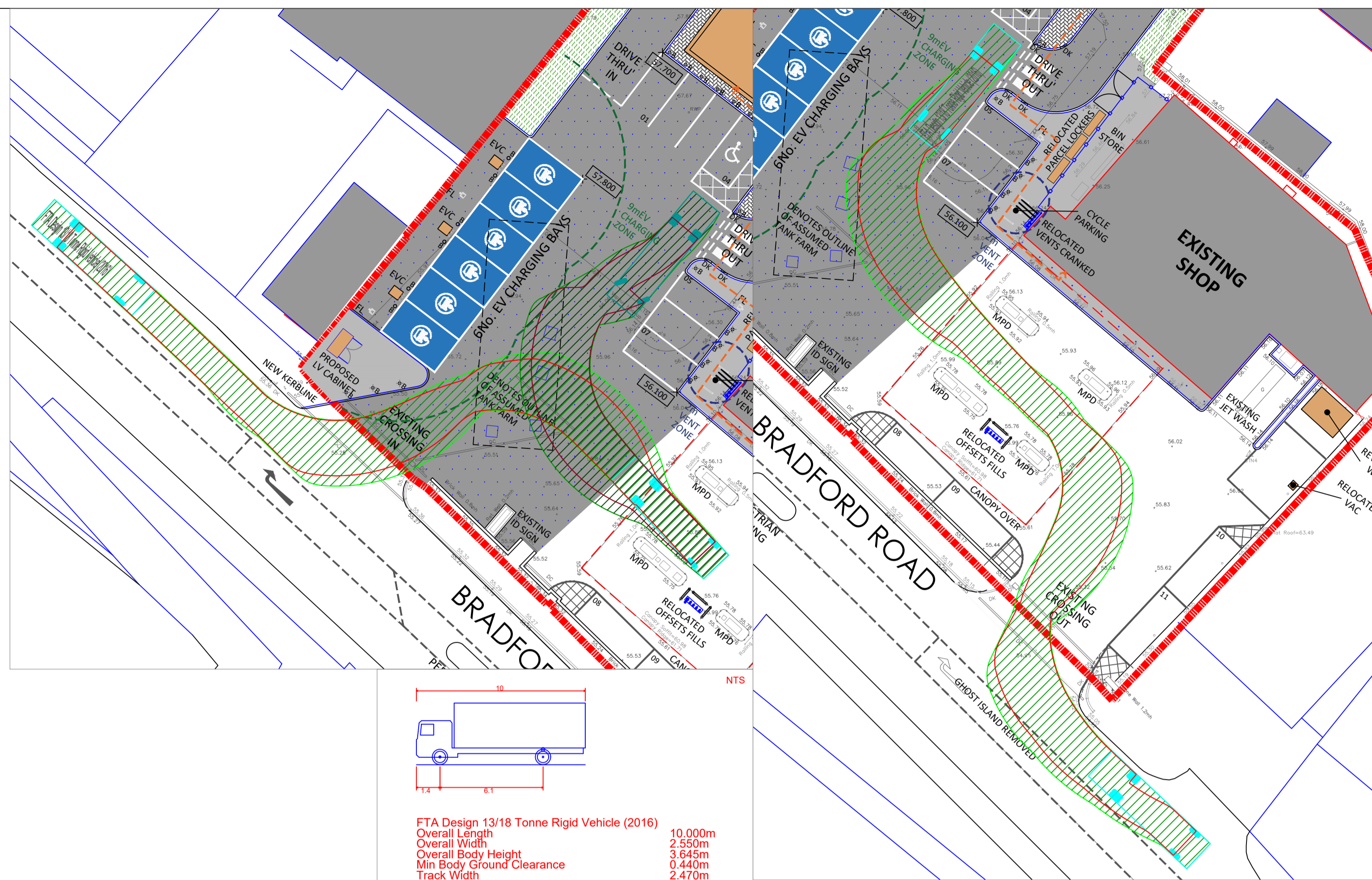
Swept Path Analysis - 10m Rigid - Scale 1/250
