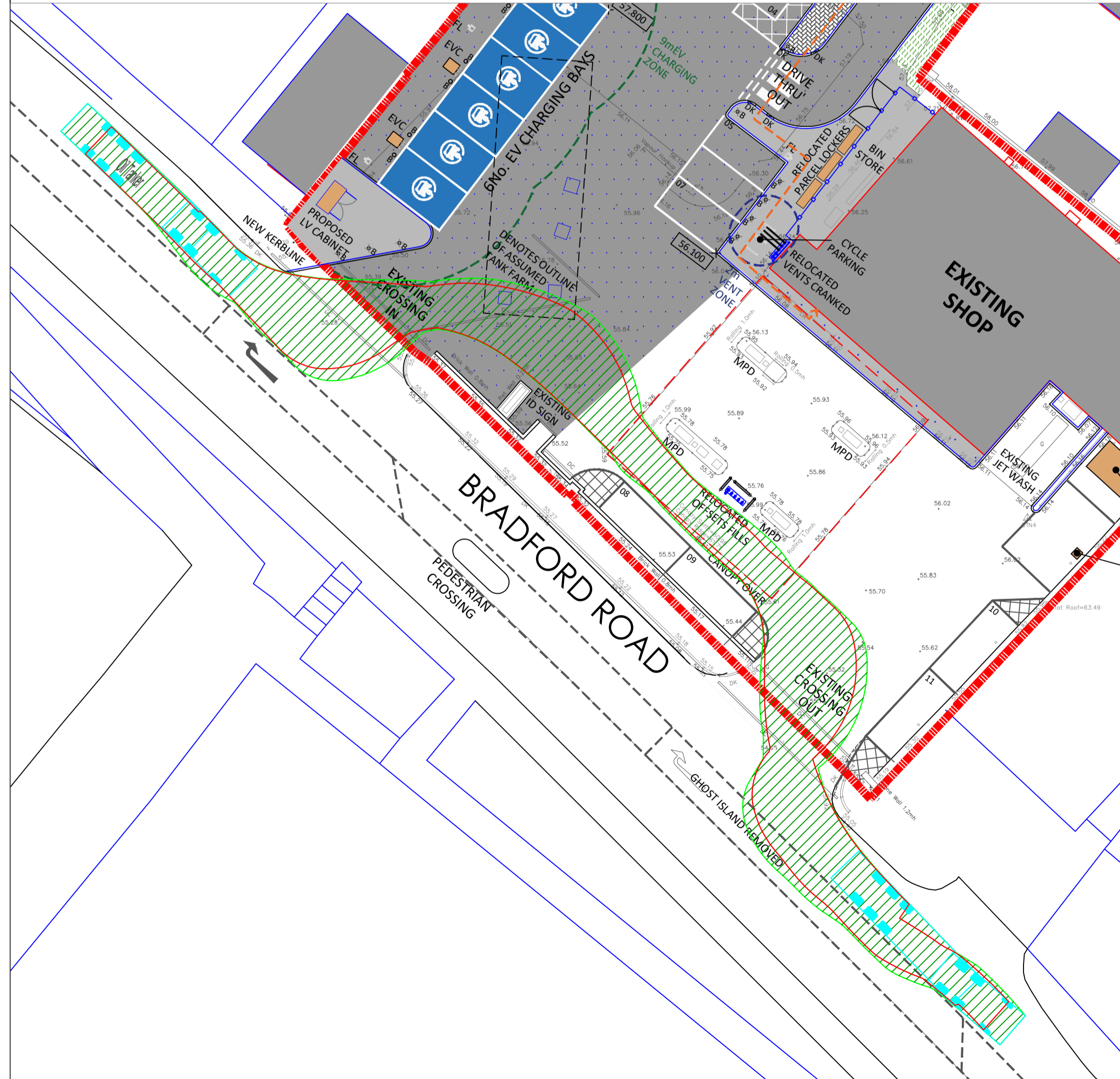
Swept Path Analysis - Oil Tanker - Scale 1/250
