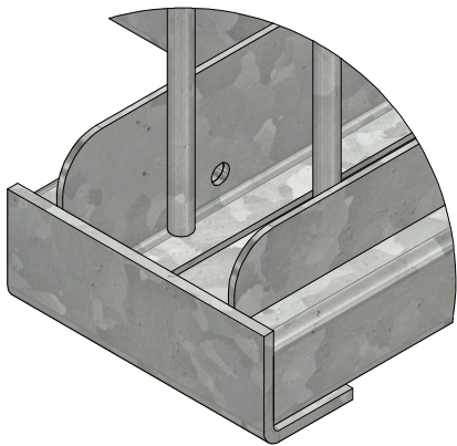
IMPROVED END PLATE Y ( 1:3 )
