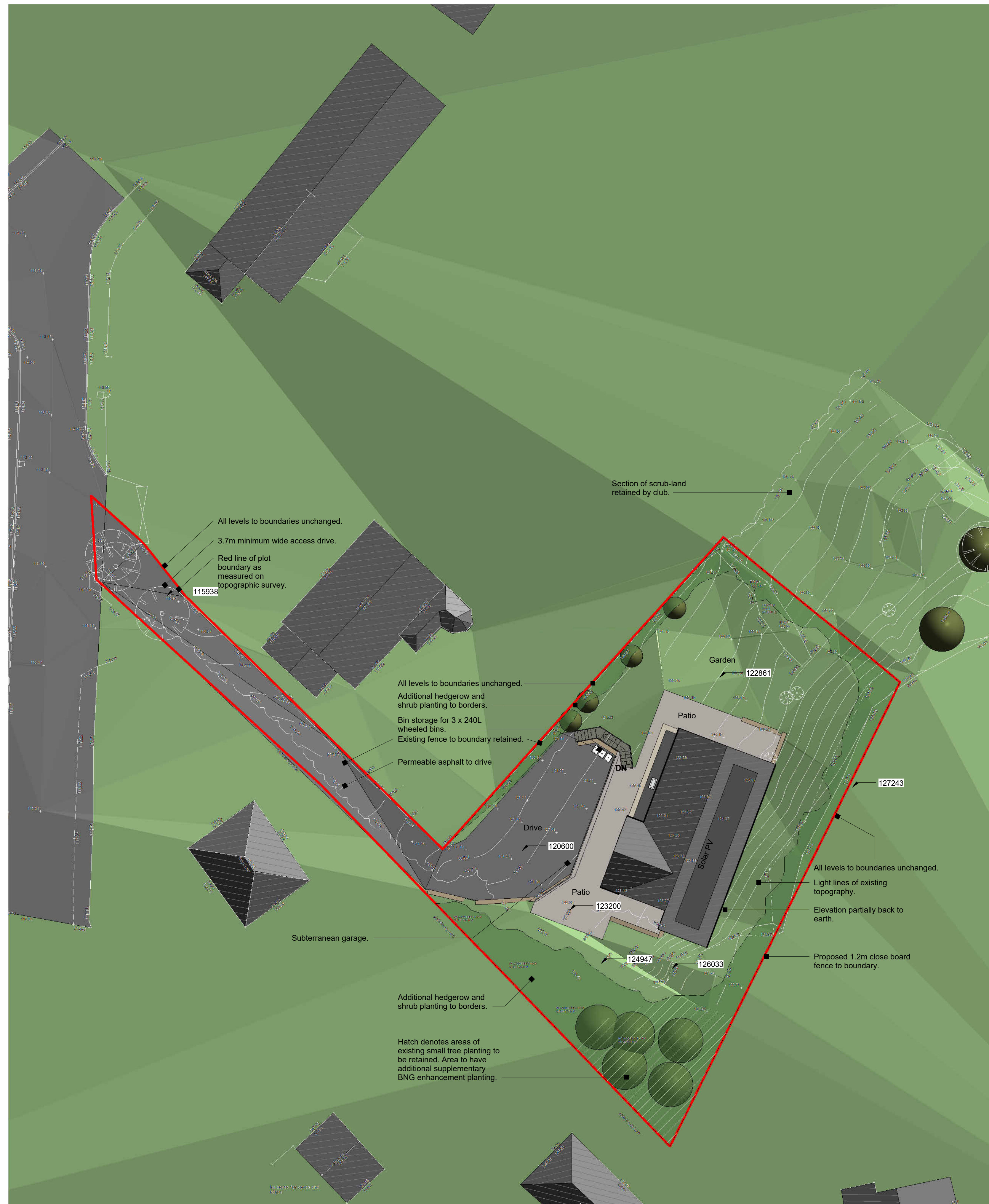
Proposed Site Plan 1:200
