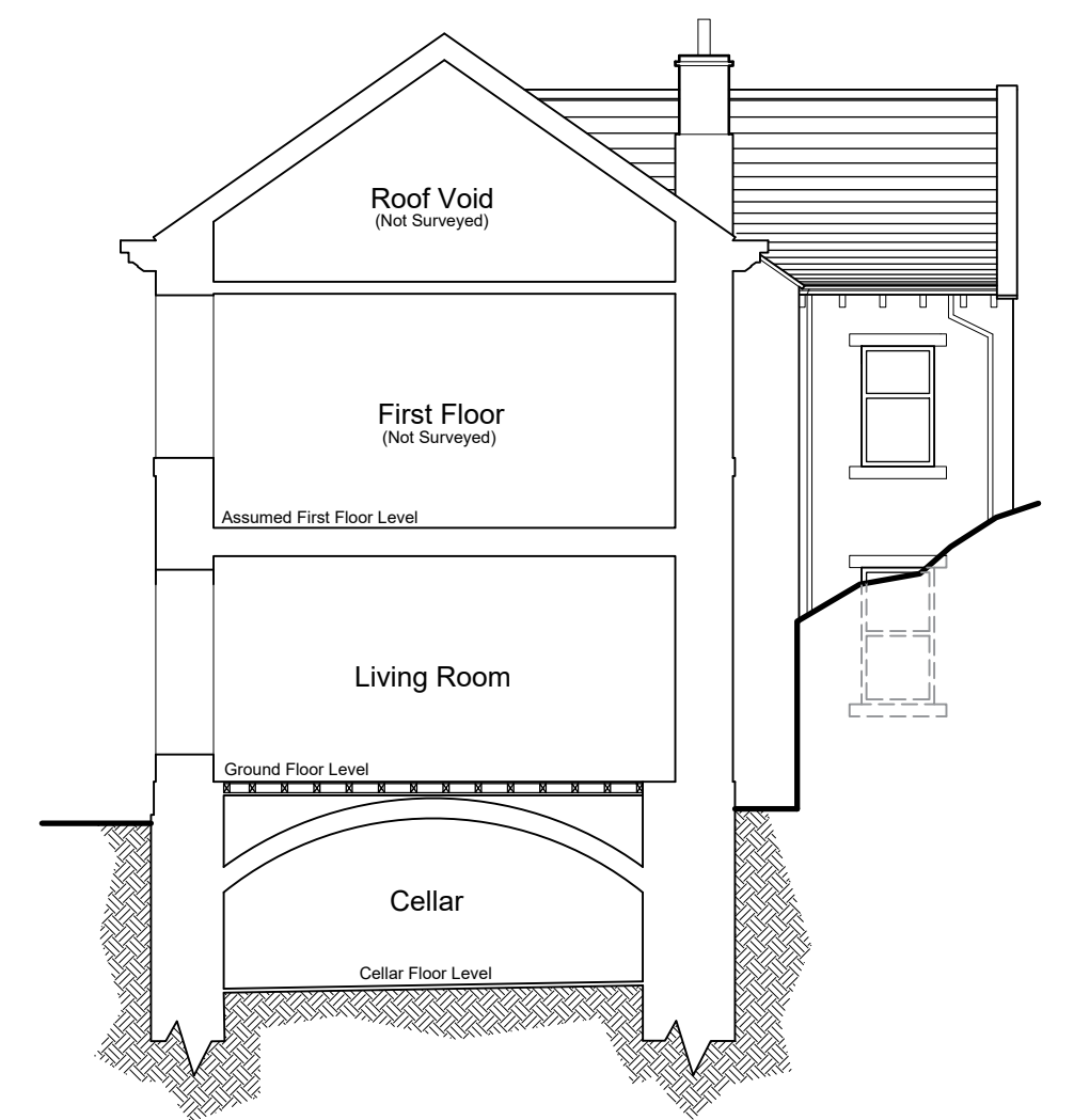
Section B-B
