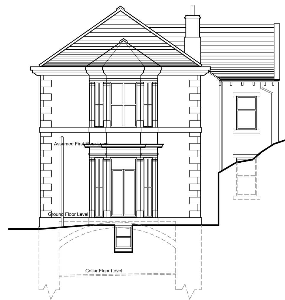
North East Elevation (side)
