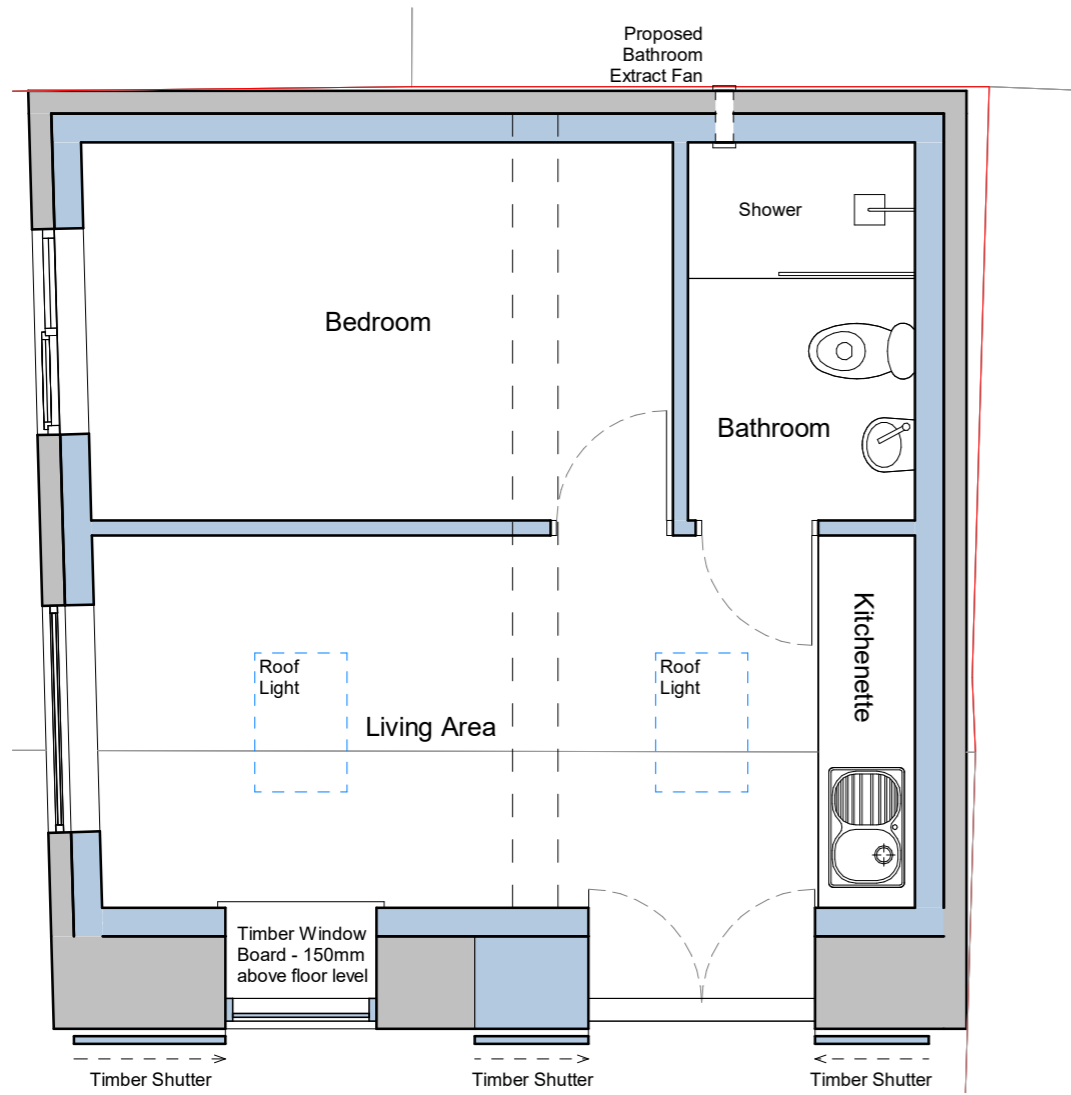
Proposed Ground Floor GA Plan
