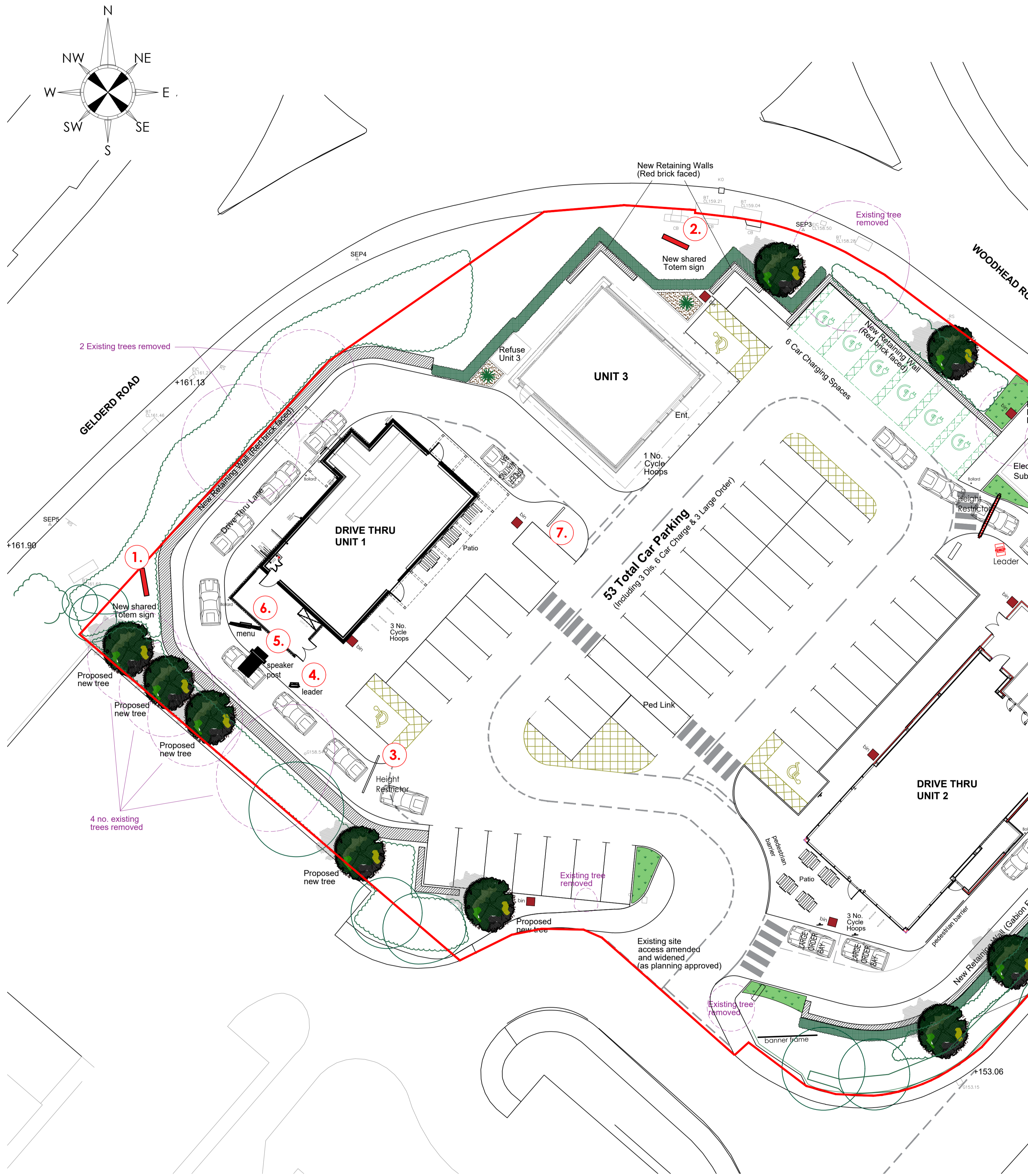
Proposed site signage plan scale - 1:200 @ A1 / 1:400 @ A3
