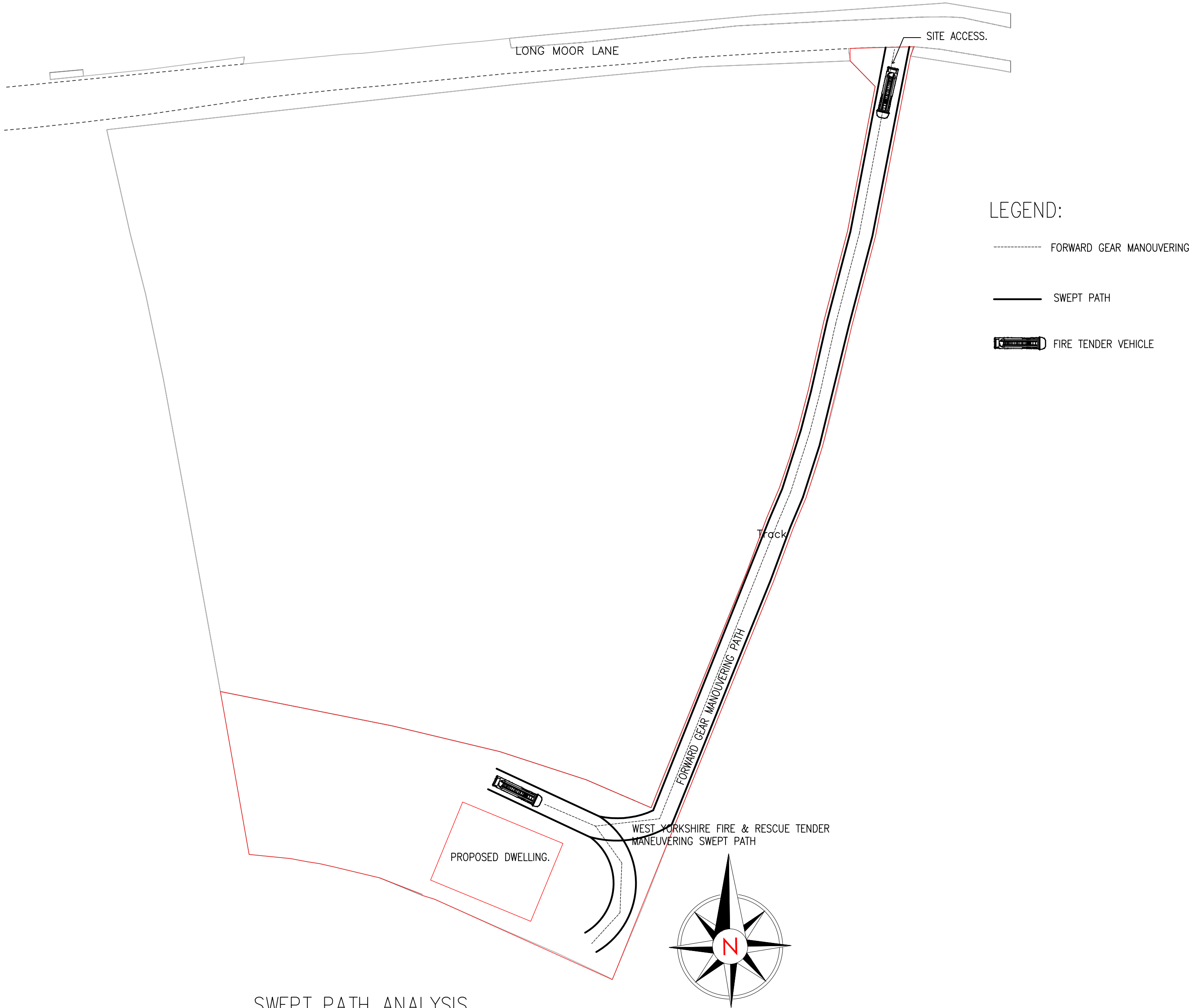
SWEPT PATH ANALYSIS. SCALE 1:200.
