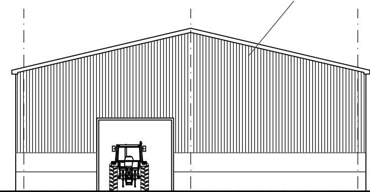
SOUTH ELEVATION
