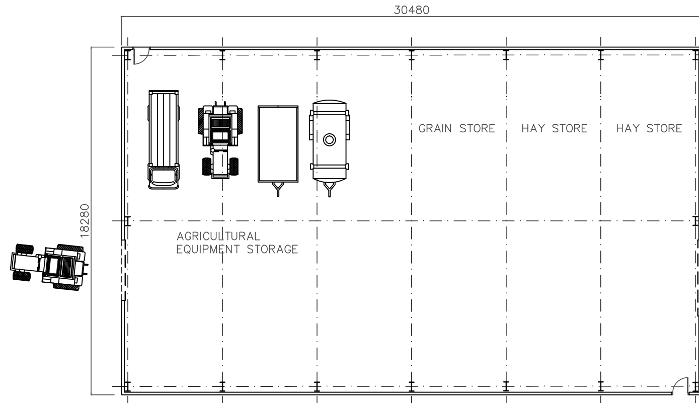
FLOOR PLAN
