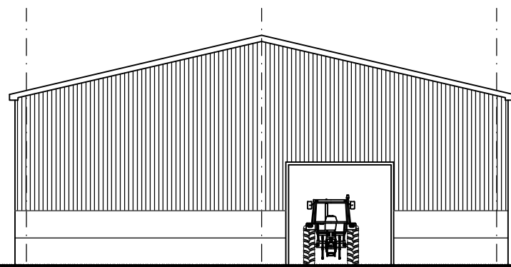
NORTH ELEVATION
