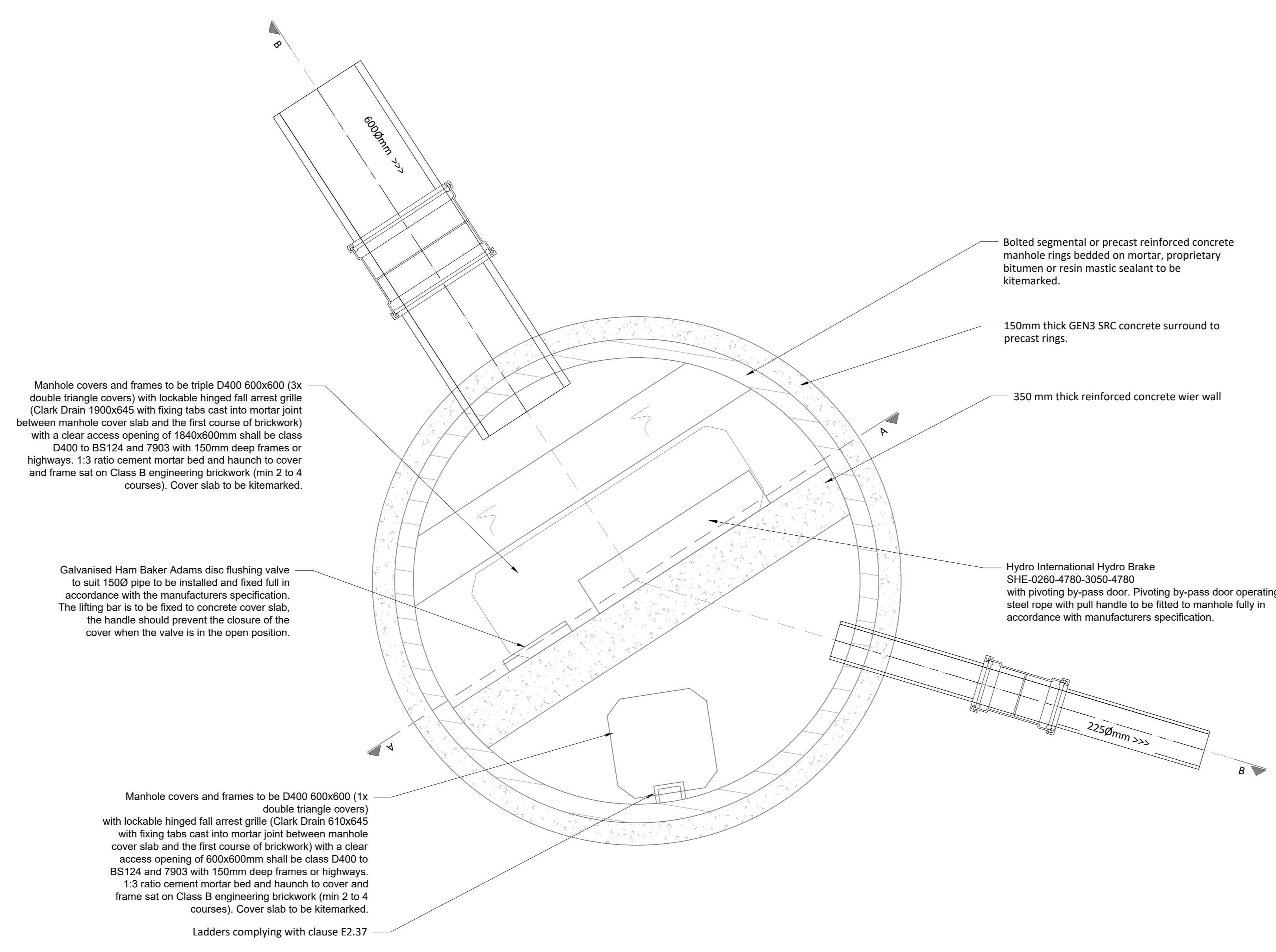
Base Plan SW73 Scale 1:20
