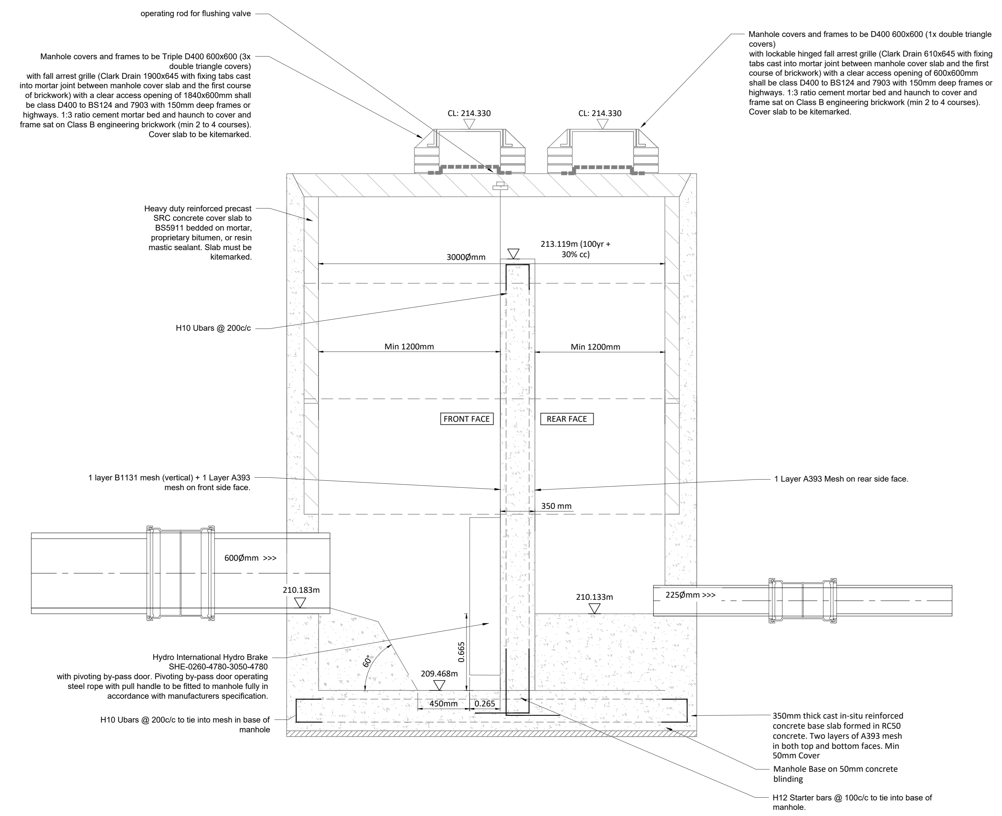
Section B-B Scale 1:20
