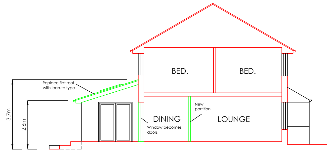
PROPOSED SECTION A-A / SIDE ELEVATION (NE)
