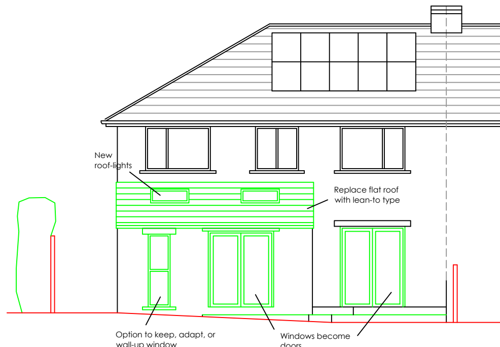
PROPOSED REAR ELEVATION (SE)
