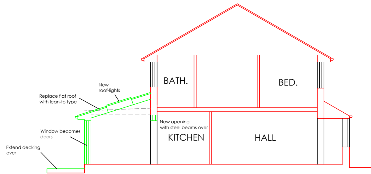
PROPOSED SECTION B-B
