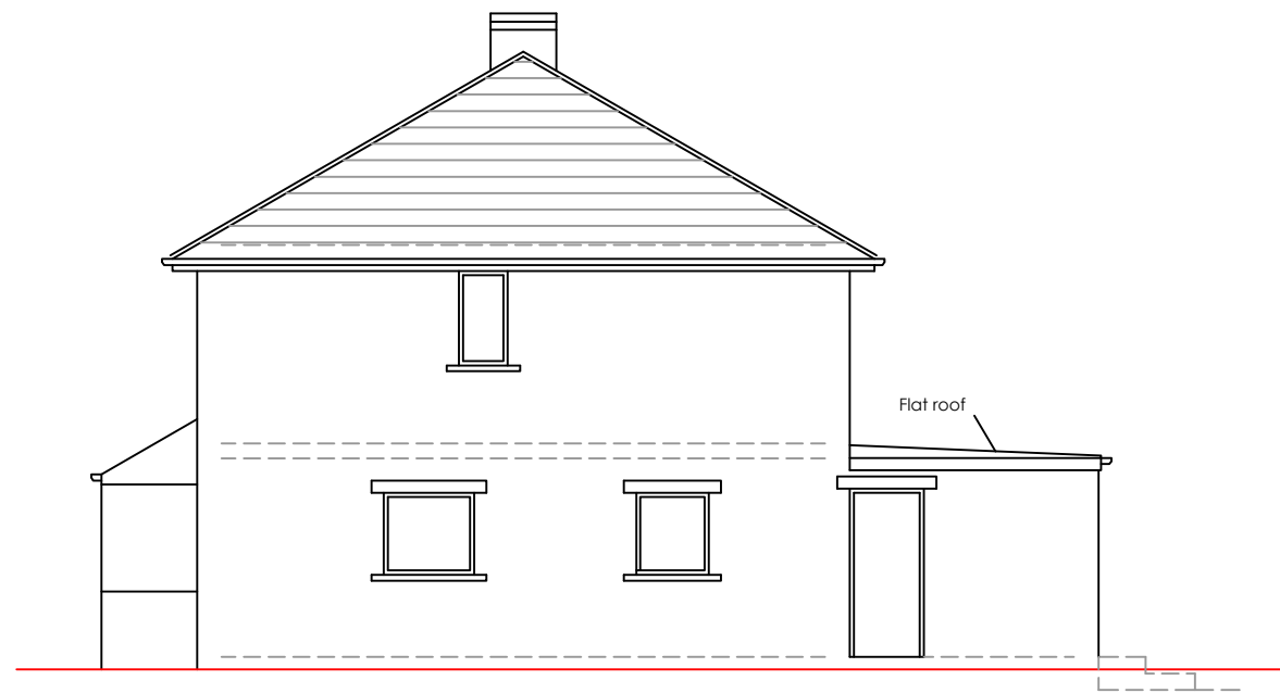
EXISTING SIDE ELEVATION (SW)
