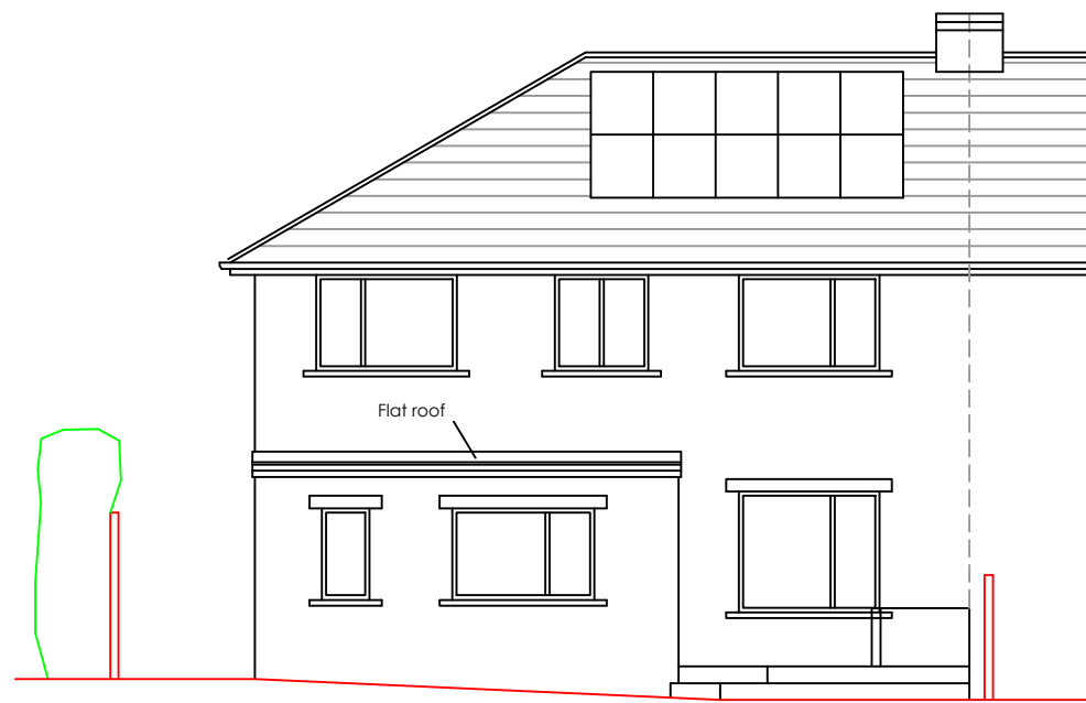
EXISTING REAR ELEVATION (SE)
