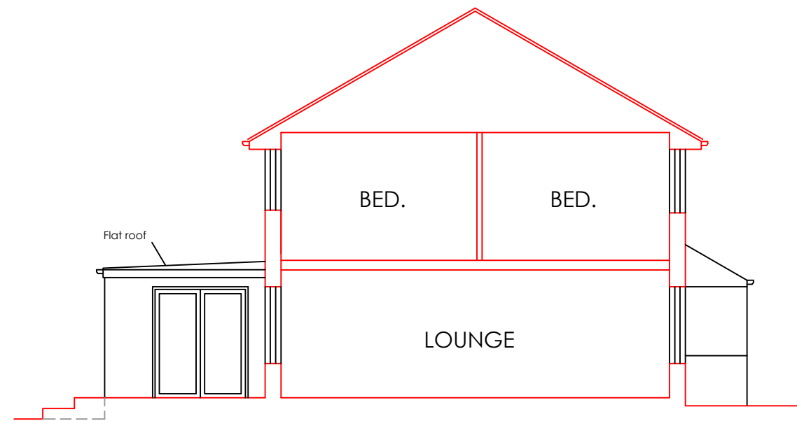
EXISTING SECTION A-A / SIDE ELEVATION (NE)
