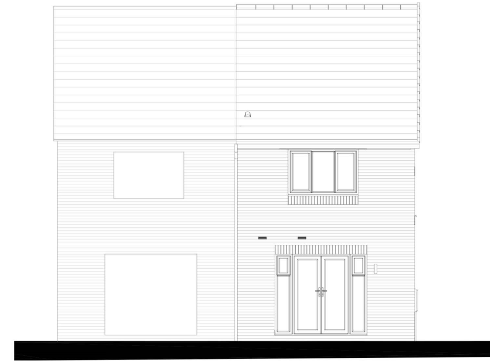
REAR ELEVATION
