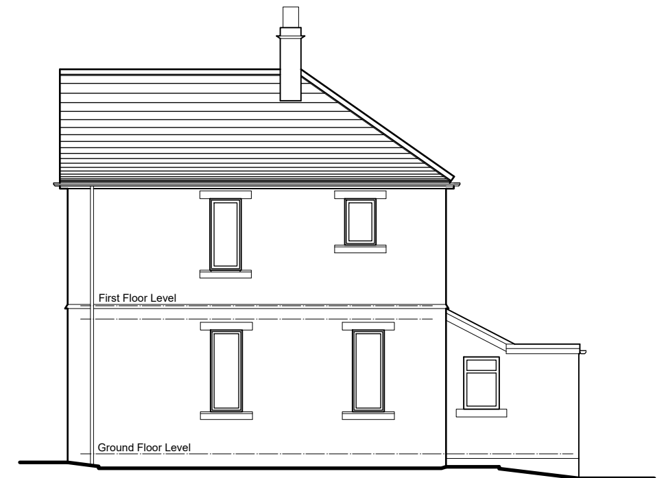
East Elevation (side)
