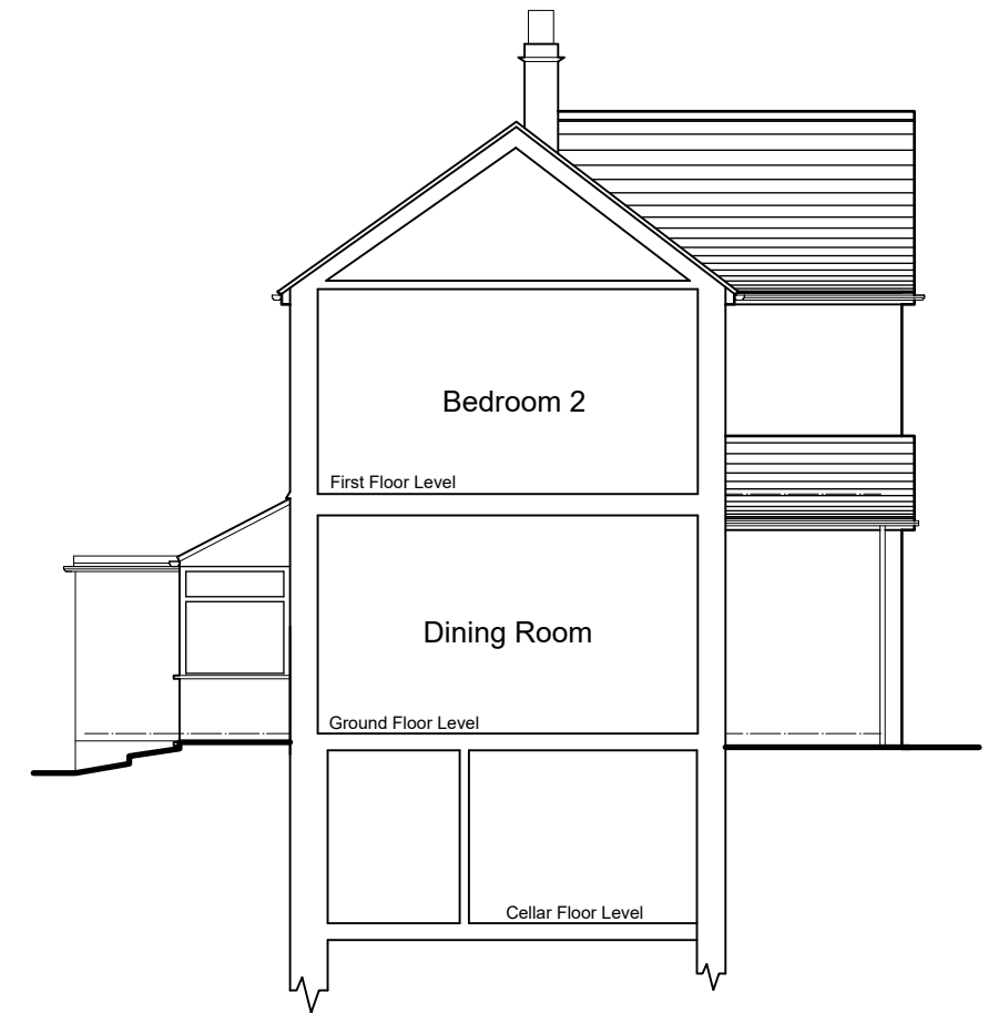
West Sectional Elevation ( Party Wall) (side)
