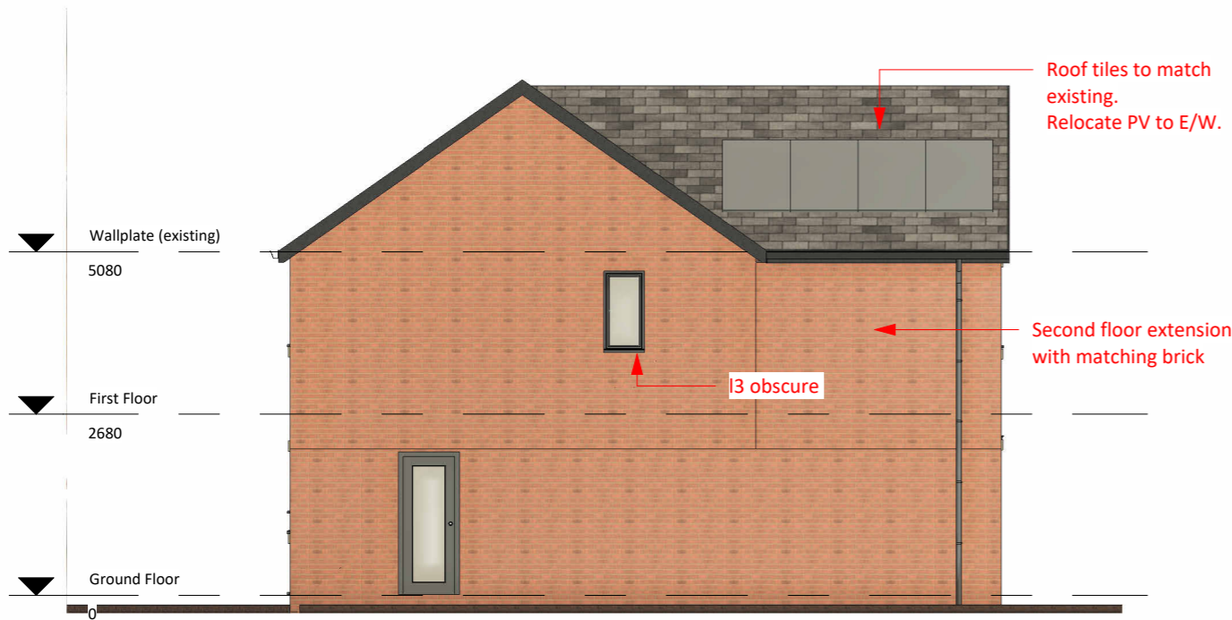
3 11 Proposed West Elevation 1 : 100
