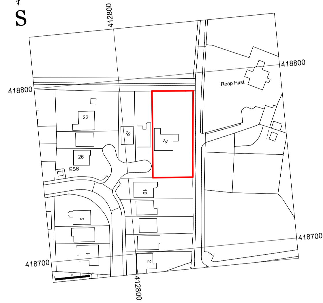
Location Plan 1 : 1250
