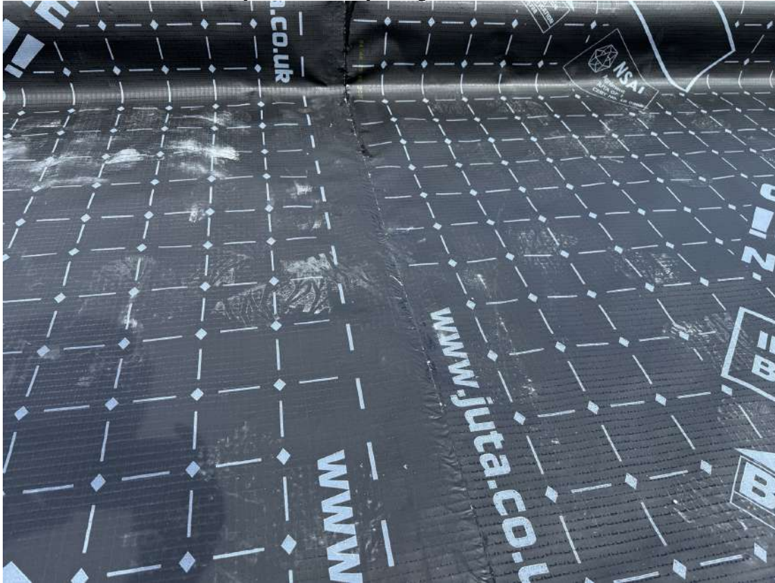
Plot 155-158 – Membrane layout with tophats and jointing
