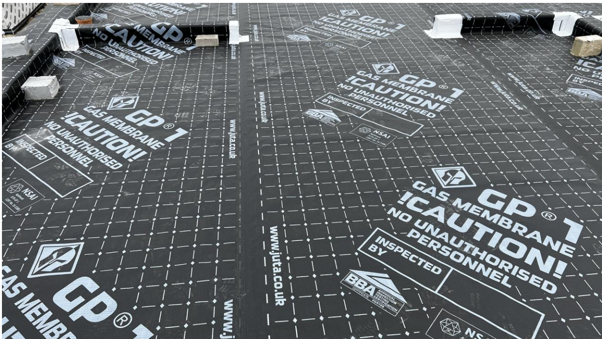
Plot 83 – Membrane layout with weld joint and internal walls.
