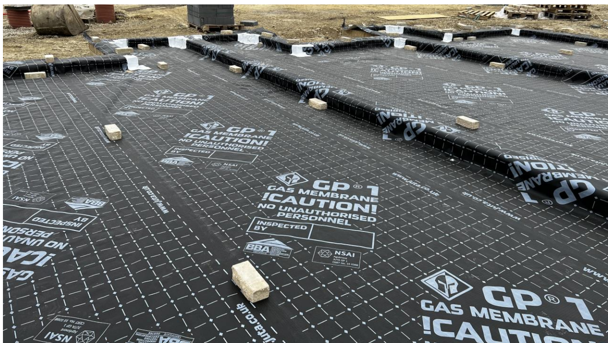
Plots 85-87 – Overall membrane layout
