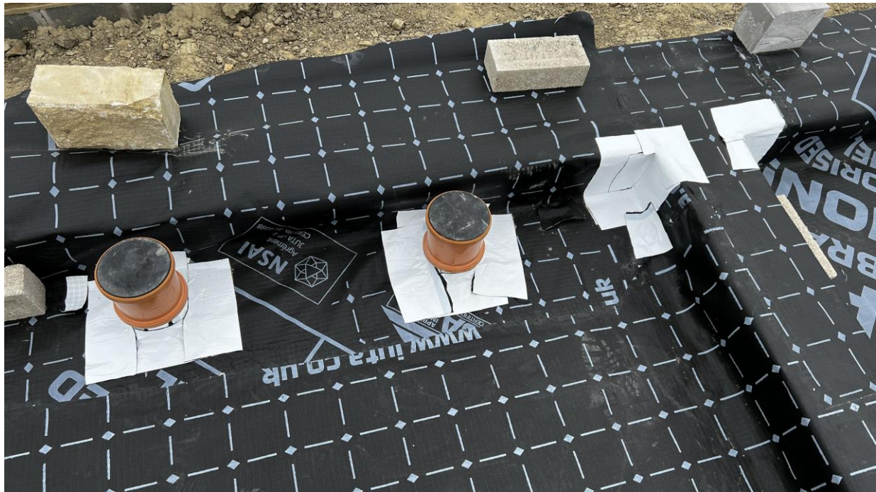
Plot 84 - Membrane layout with internal walls and weld
