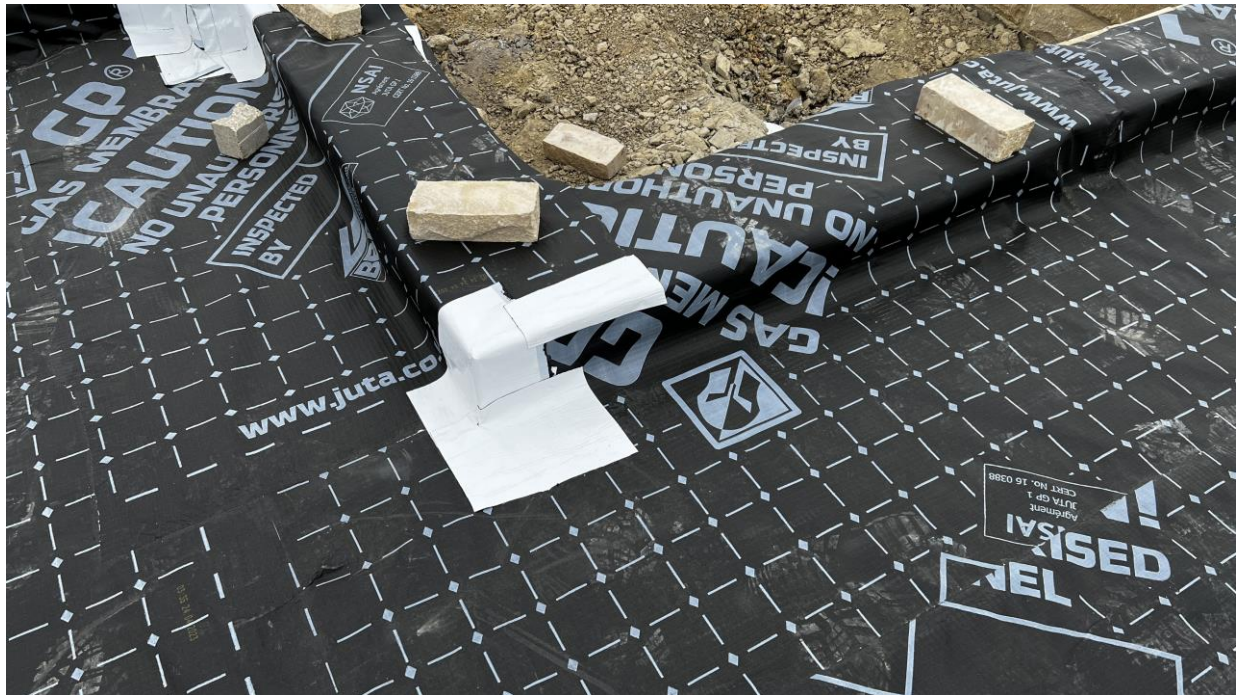
Plots 85-87 - Membrane layout with internal walls, jointing and a tophat
