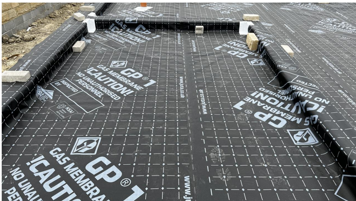
Plot 84 - Membrane layout with internal walls and weld
