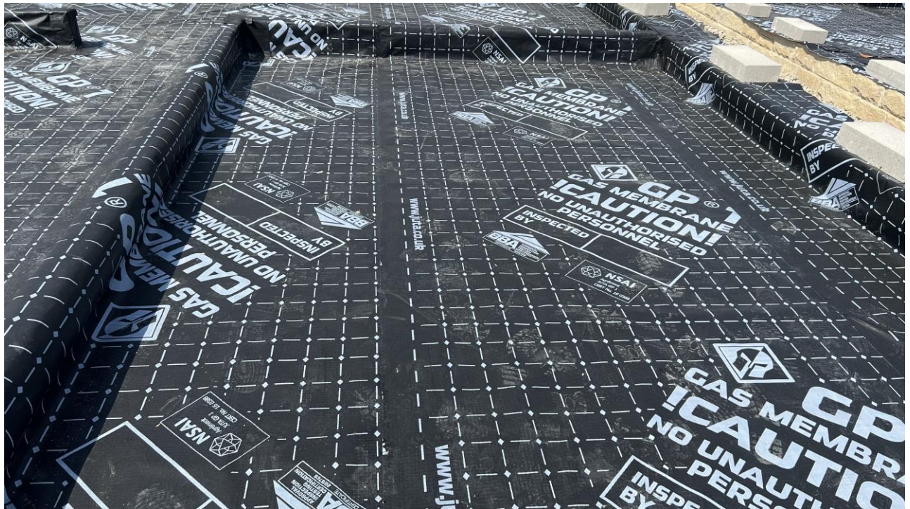
Plot 120 – Overall membrane layout
