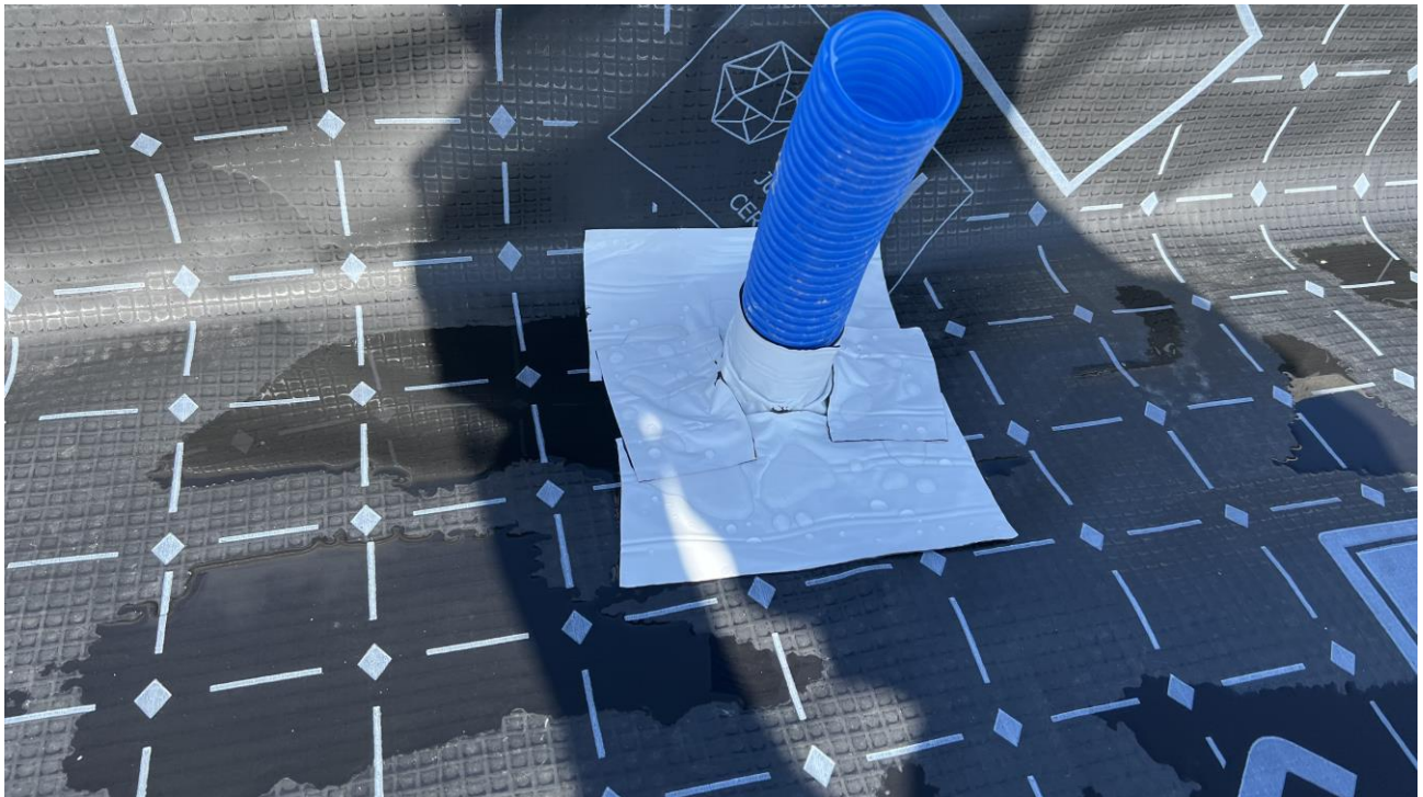
Plots 121 & 122 – Membrane layout with tophat and jointing
