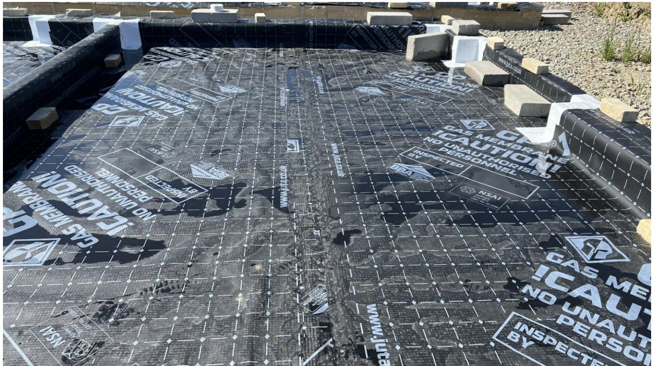
Plot 124 – Membrane layout with weld joint and internal wall
