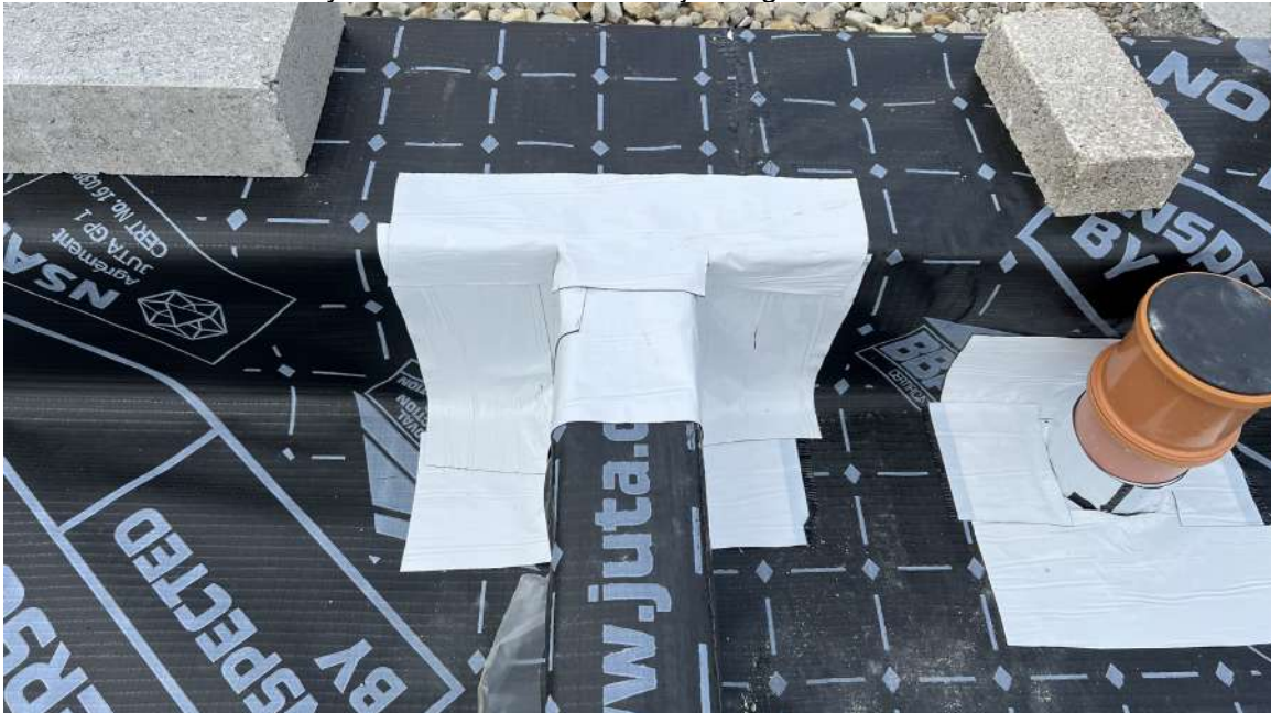
Plot 110 – Membrane layout with internal wall and jointing
