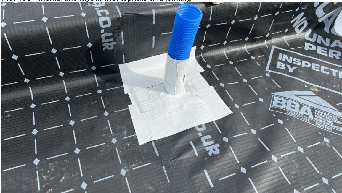
Plot 108 - Membrane layout with tophats and jointing
