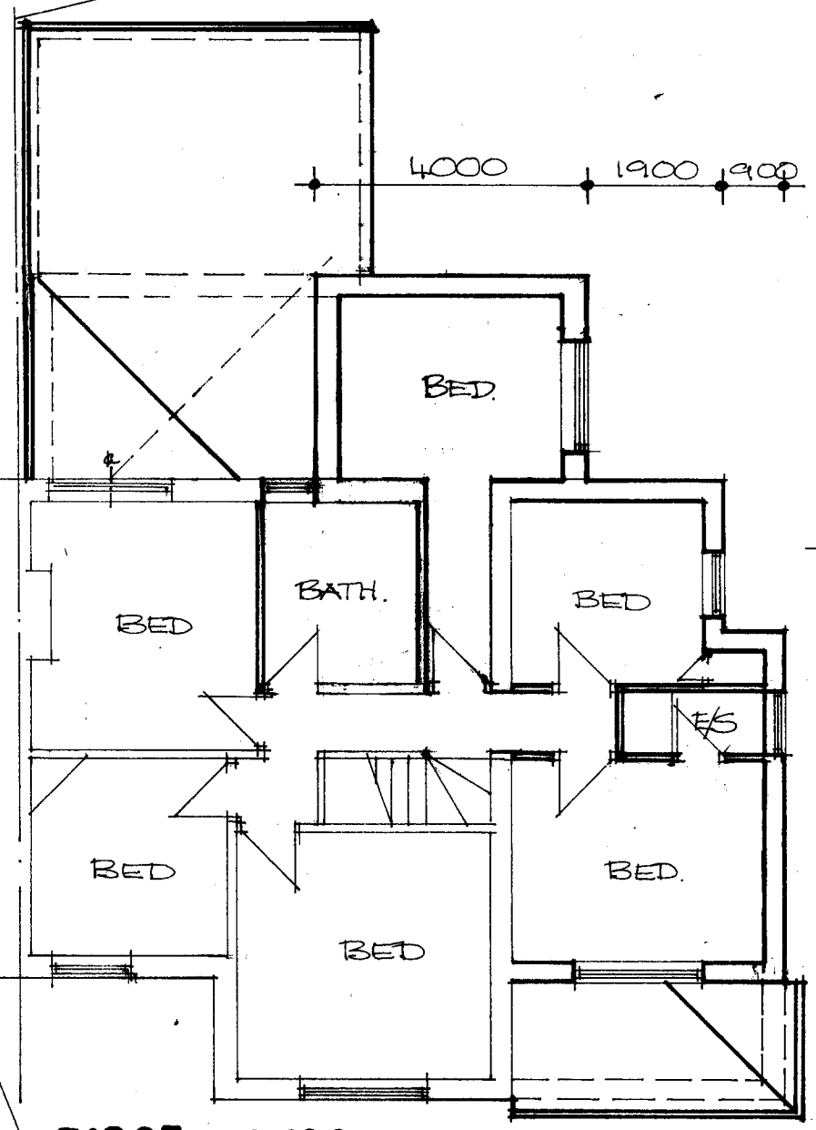
FIRST 1:100
