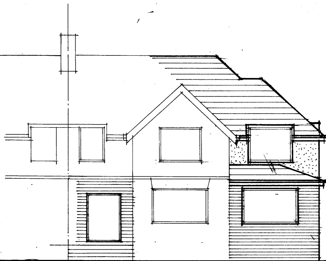
FRONT 1:100
