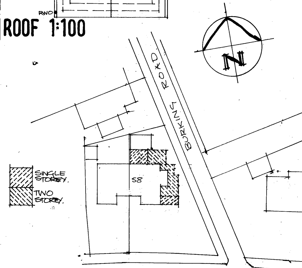
BLOCK PLAN 1:500
