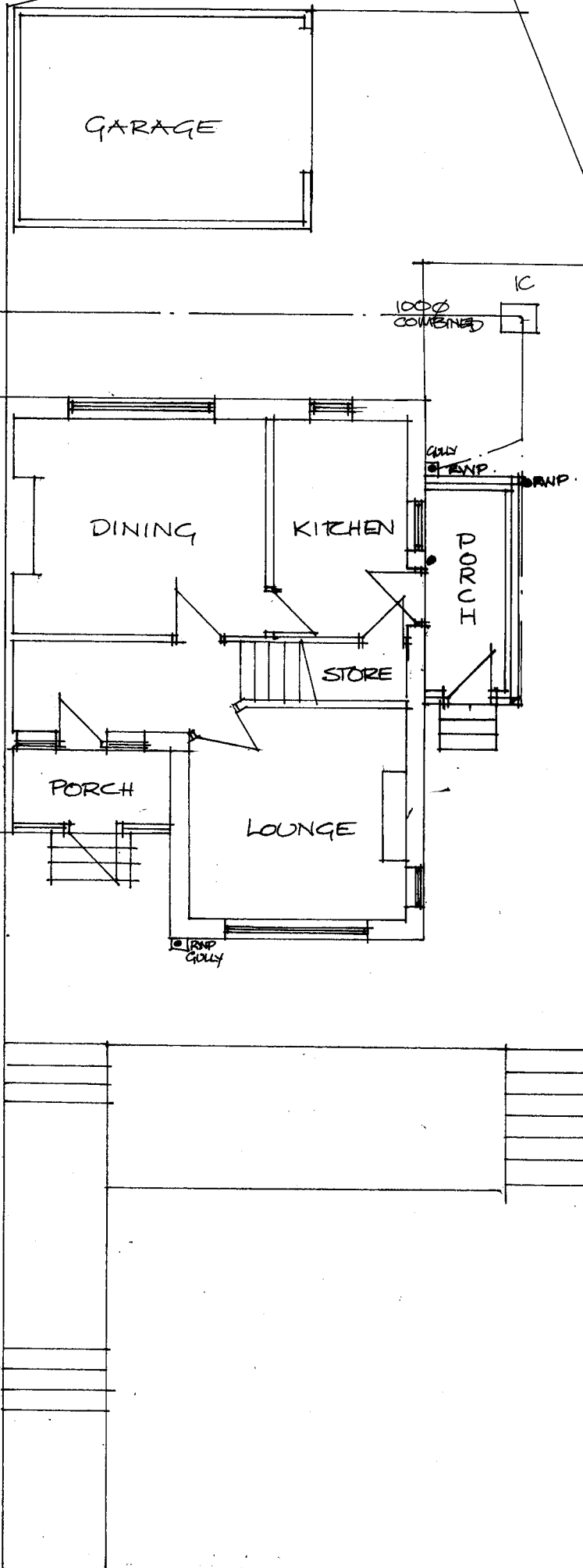
GROUND 1:100
