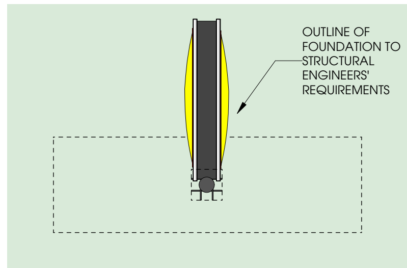
FLAGPOLE SIGNAGE PLAN VIEW 1:50
