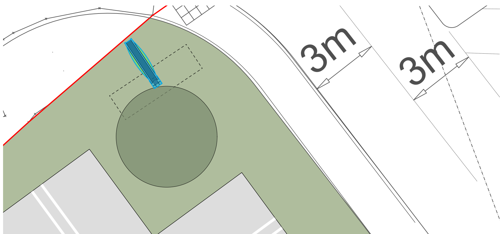
FLAGPOLE LOCATION 1:100
