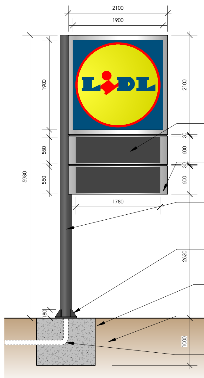
FLAGPOLE SIGNAGE FRONT ELEVATION 1:50
