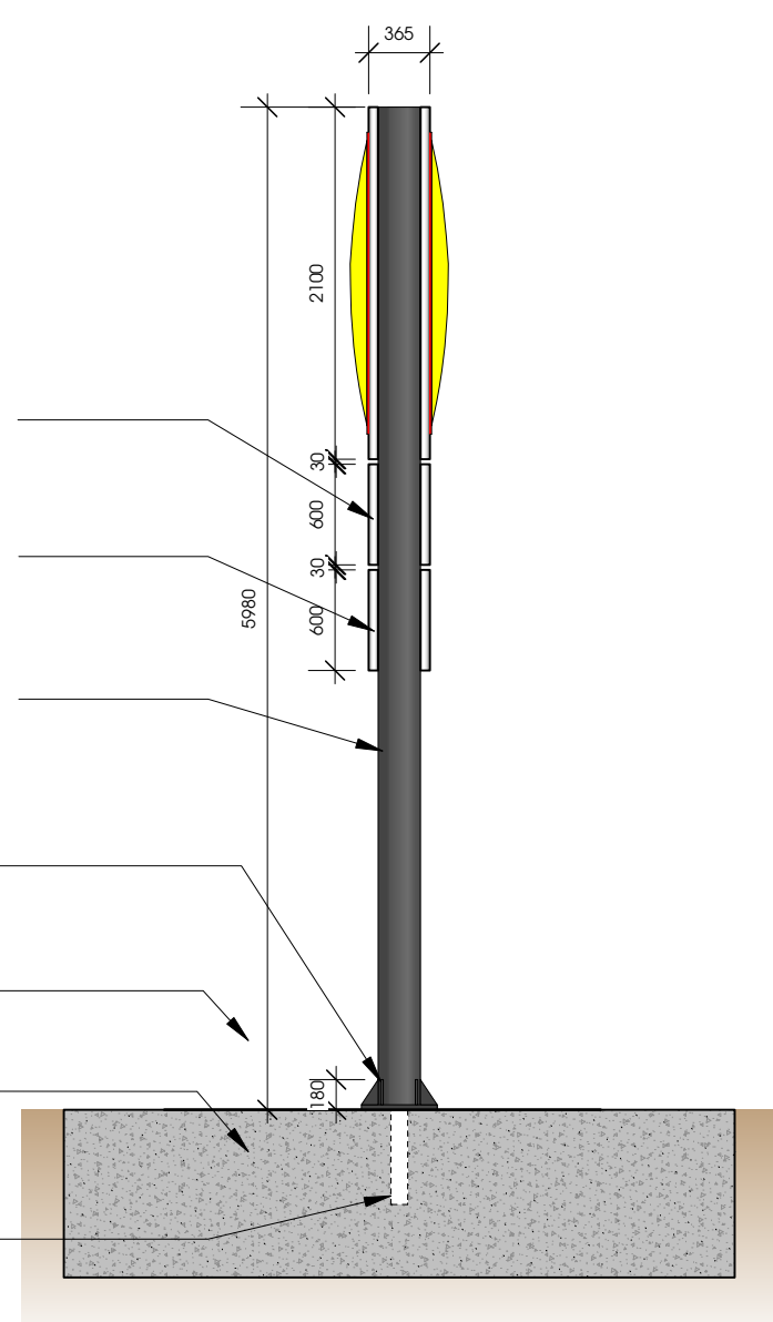
FLAGPOLE SIGNAGE SIDE ELEVATION 1:50
