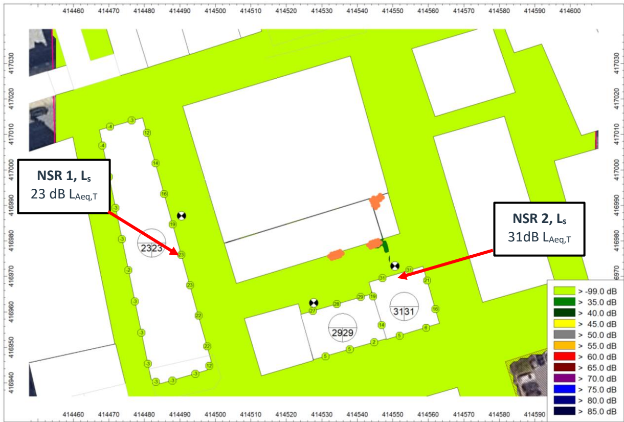
Figure 4: Sound contours at 3 m, showing the night time calculated specific plant sound level, L_{Aeq, 15 \text{ min}} (with mitigation)
