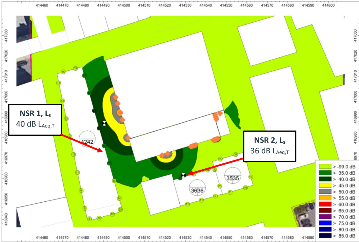
Figure 3: Sound contours at 3 m, showing the daytime calculated specific plant sound level, L_{Aeq\ 1\ hr} (with mitigation)
