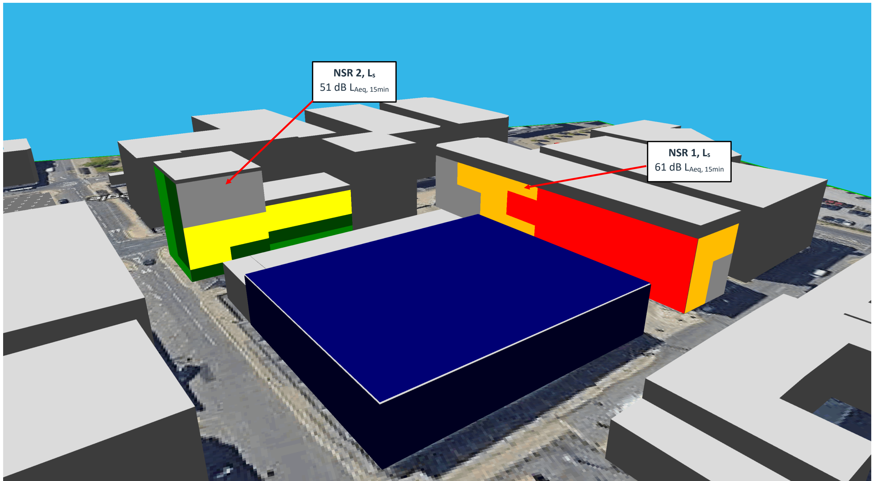
Figure 5: Building sound contours, showing the calculated MNLS, L_{Aeq, 15min}
