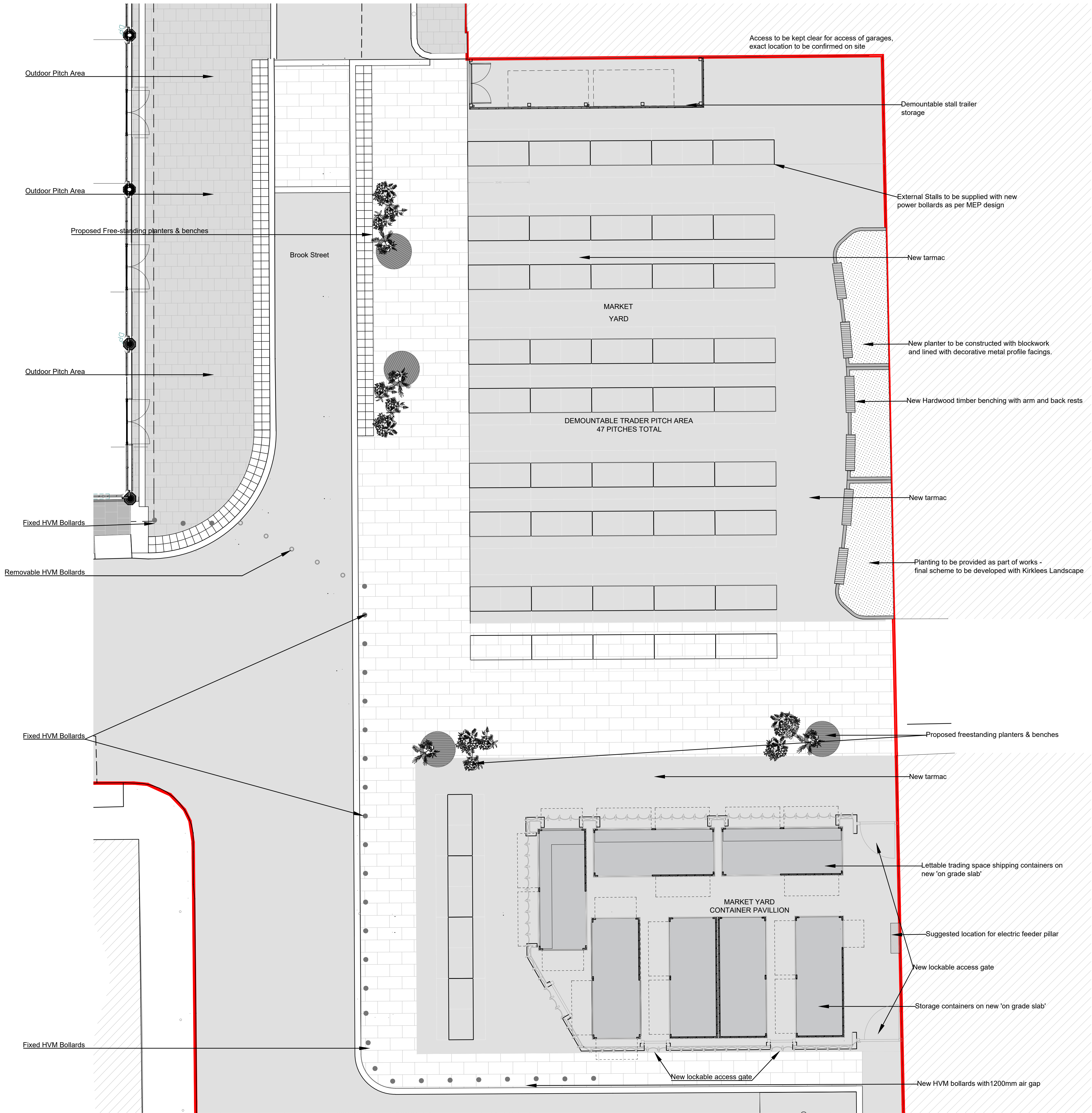
01 Market Yard Site Layout - Level 00 1:100
