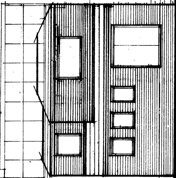
REAR 1:100
