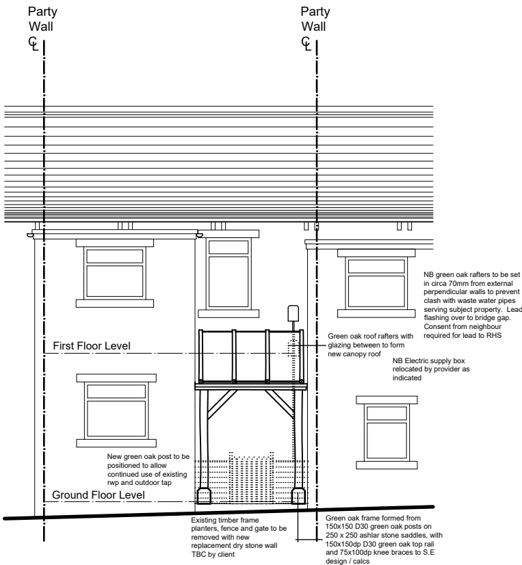
South West Elevation (front)
