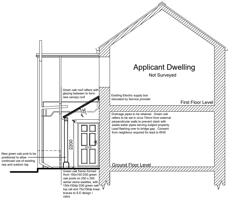
South East Sectional Party Wall Elevation (side)
