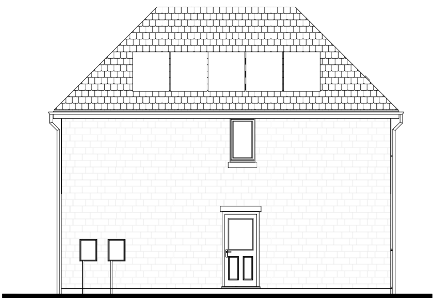
REAR ELEVATION
