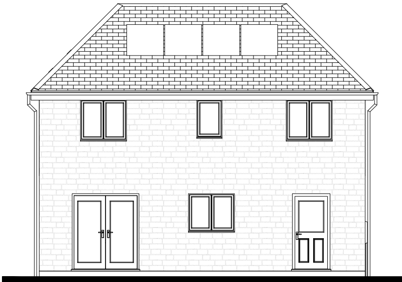
REAR ELEVATION
