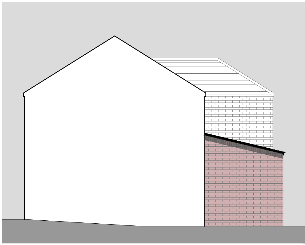
PROPOSED OTHER SIDE ELEVATION 1:100 @ A1
