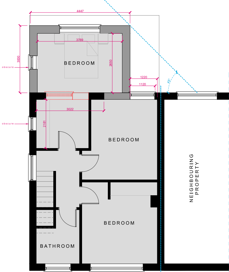
PROPOSED GROUND FLOOR PLAN 1:100 @ A1
