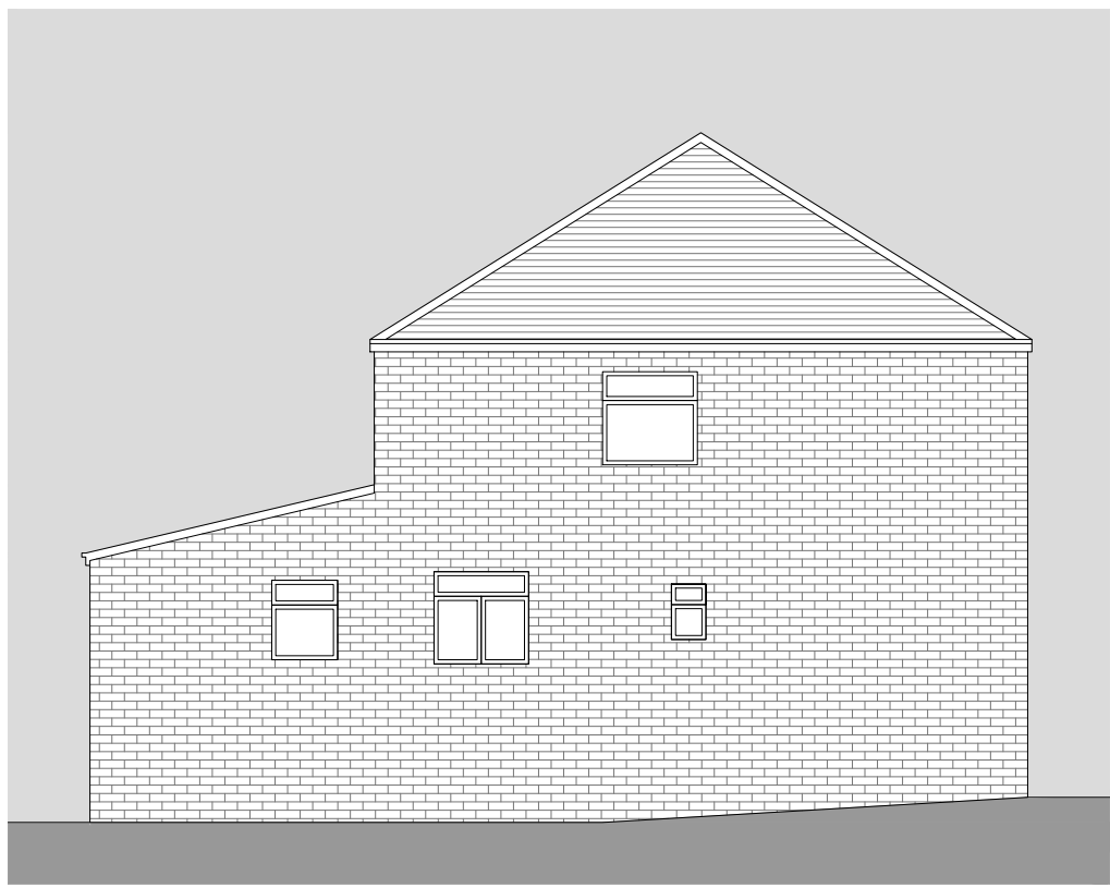
EXISTING SIDE ELEVATION 1:100 @ A1
