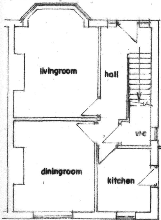
GROUND FLOOR PLAN (EXISTING)
