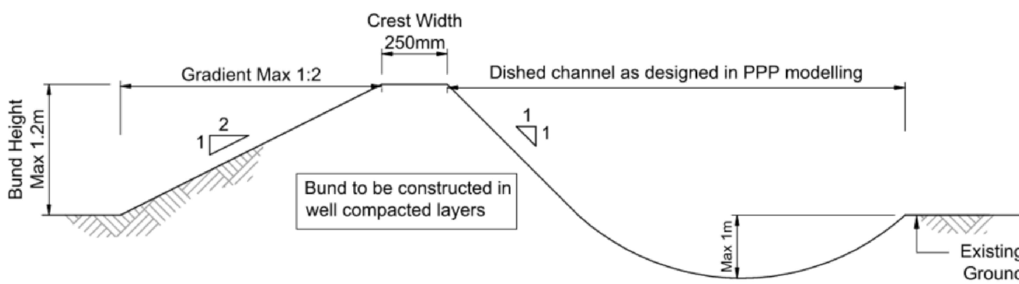
DETAIL 2 - BUND & CHANNEL (NTS)
