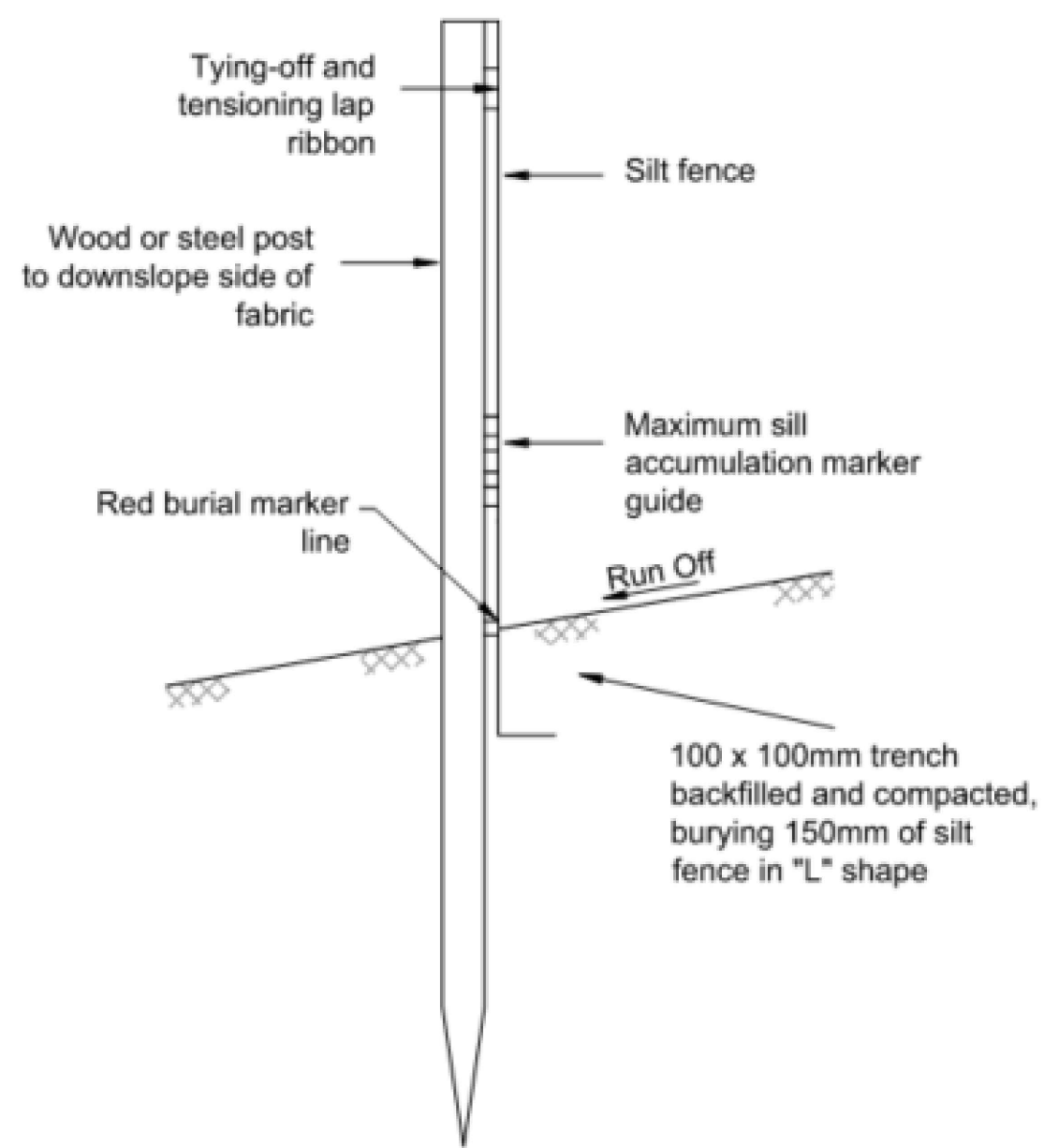
DETAIL 1 - SILT FENCING (NTS)
