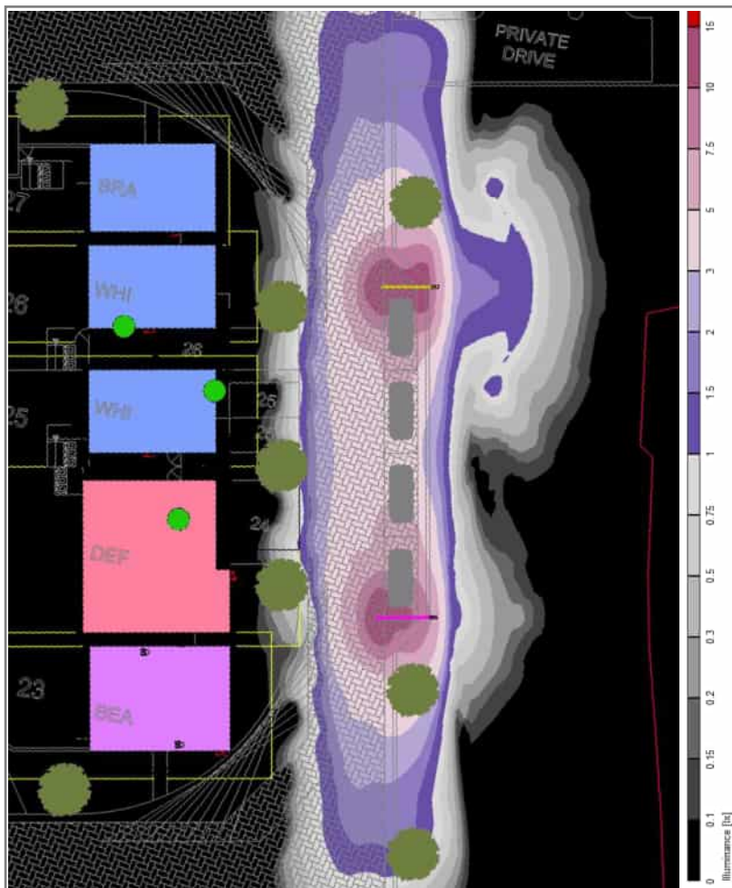
Figure 6. Unshielded vs shielded luminaires
