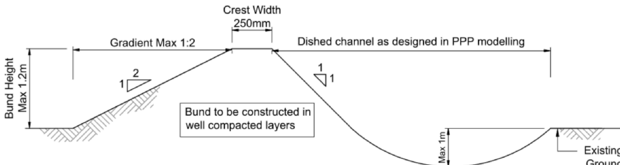
DETAIL 2 - BUND & CHANNEL (NTS)
