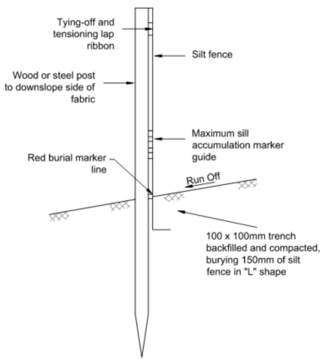
DETAIL 1 - SILT FENCING (NTS)
