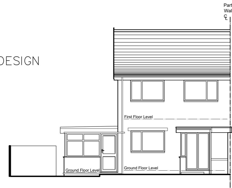
East Elevation (rear)
