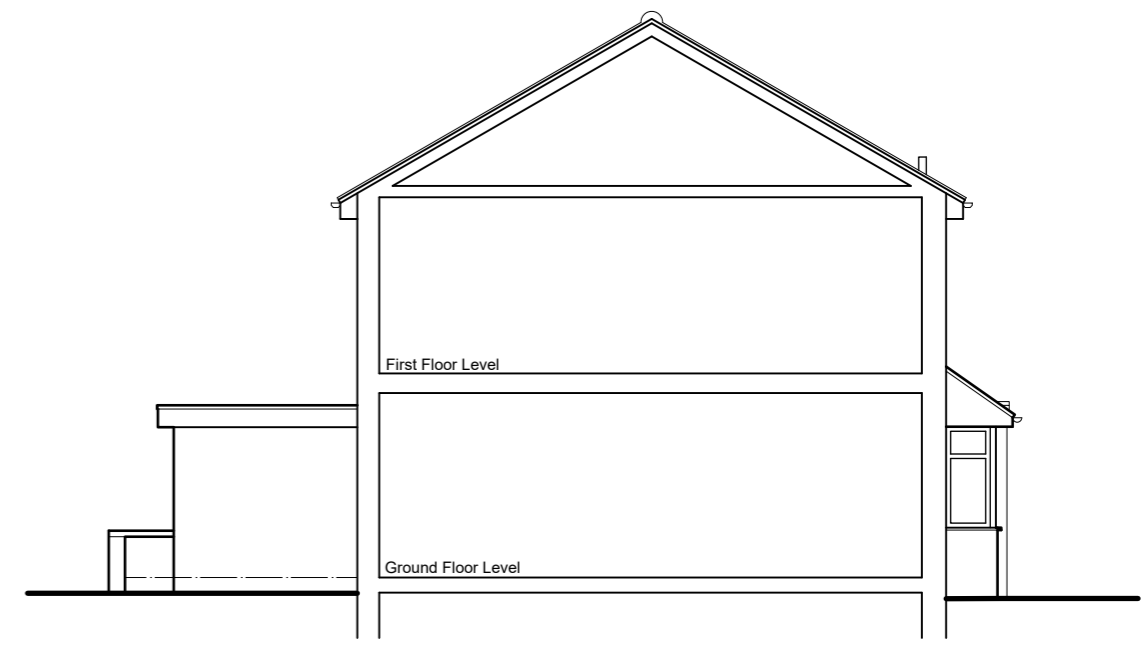
Sectional North Party Wall Elevation (side)
