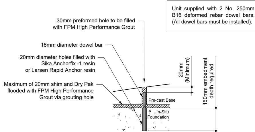
Anchor Detail Scale 1:10
