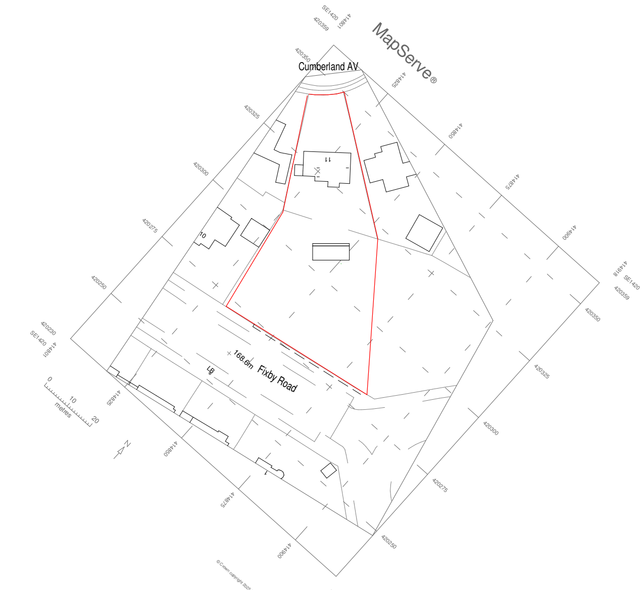
2 Location Plan 1 : 1250
