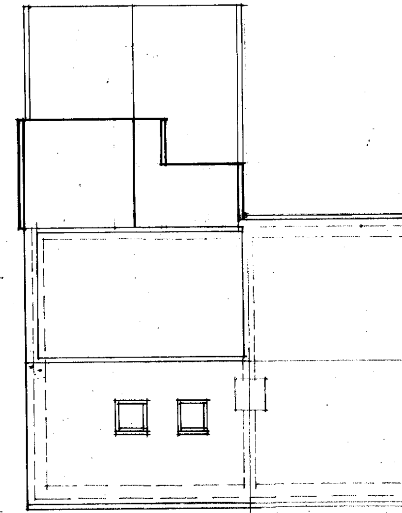
ROOF 1:100
