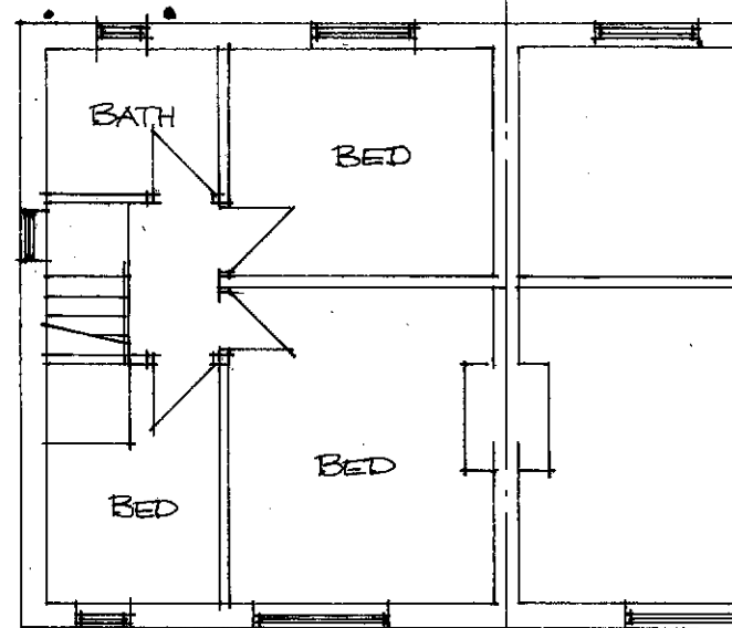
FIRST 1:100
