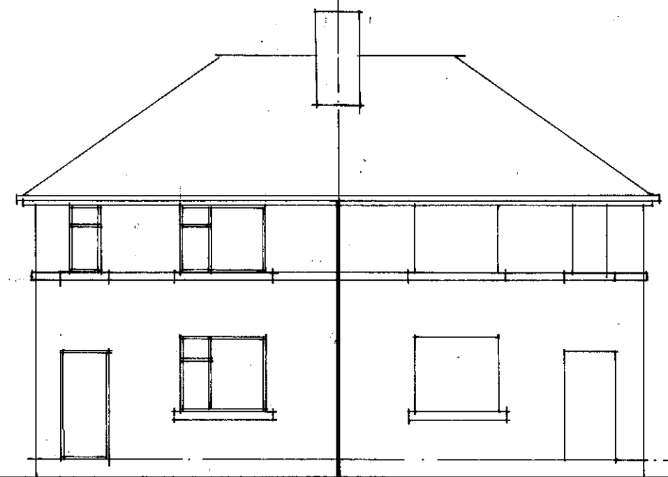
FRONT 1:100
