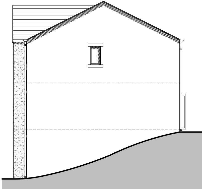
SIDE ELEVATION
