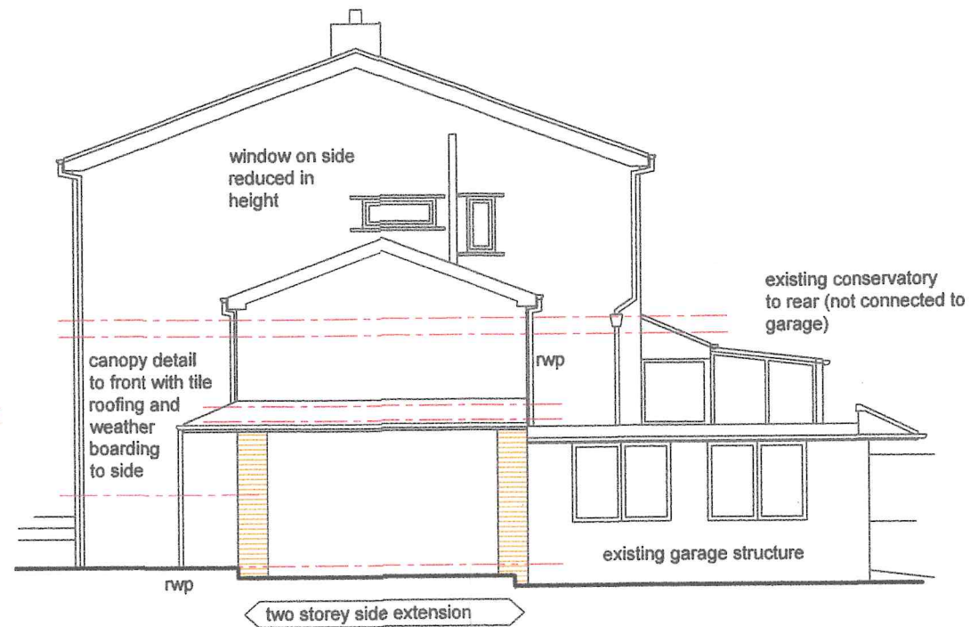
North Elevation
