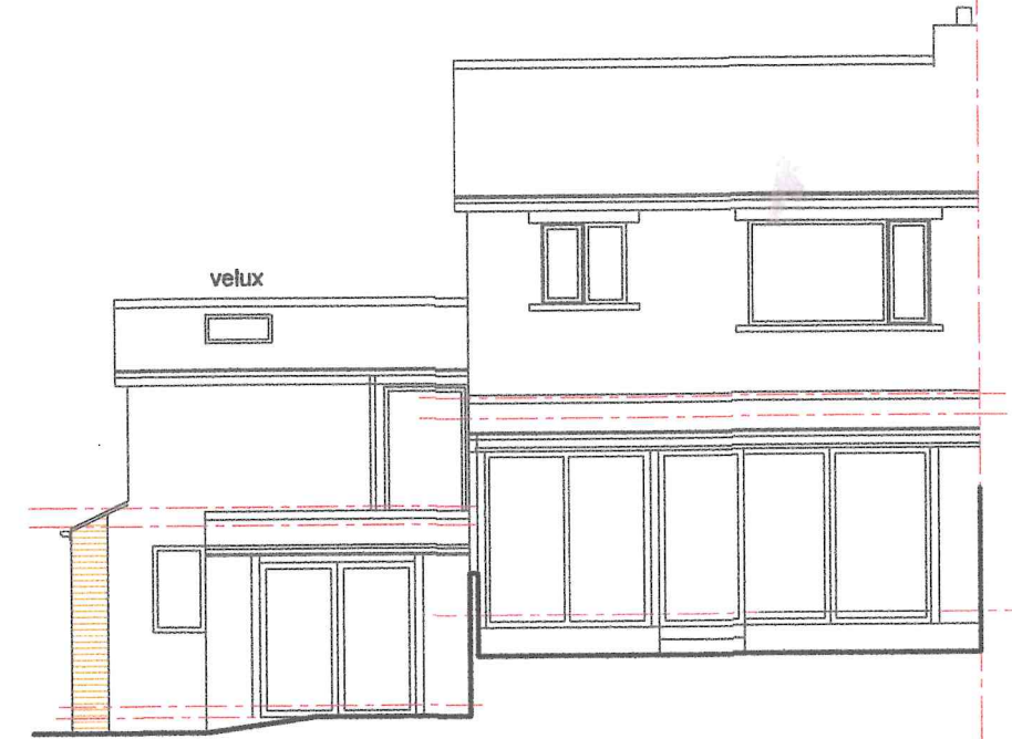
West Elevation
