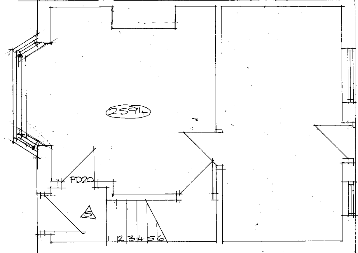
GROUND 1:50
