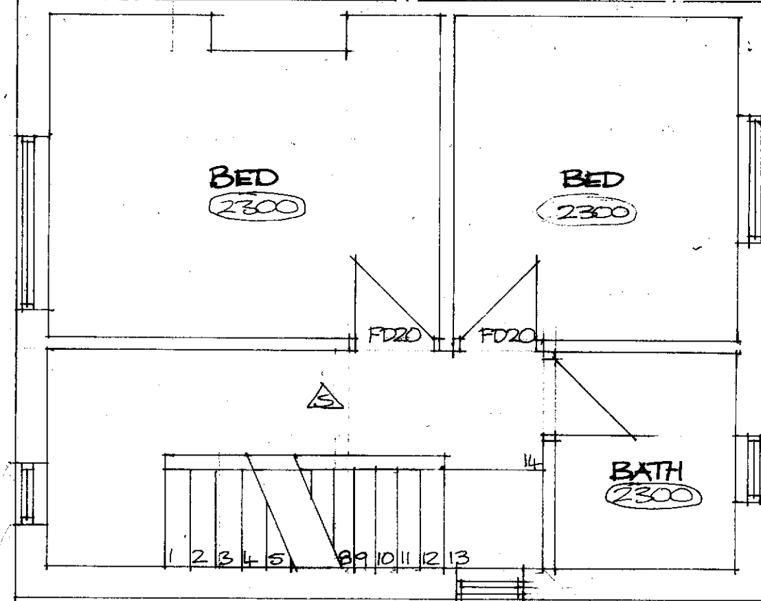
FIRST 1:50
