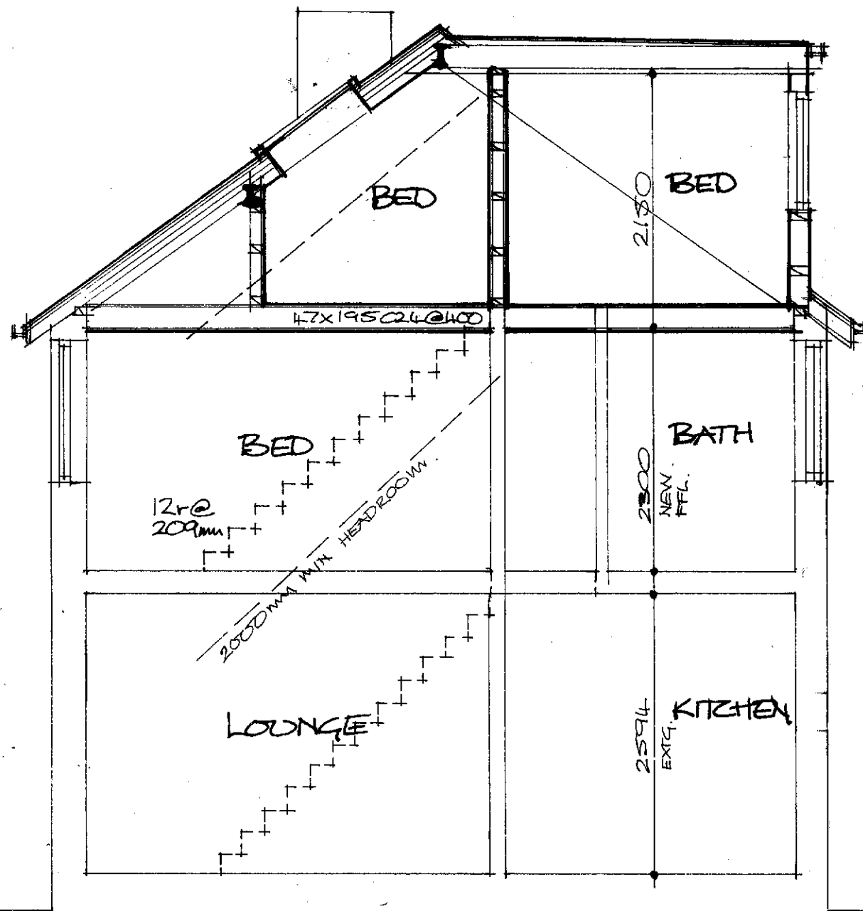
SECTION 1:50
