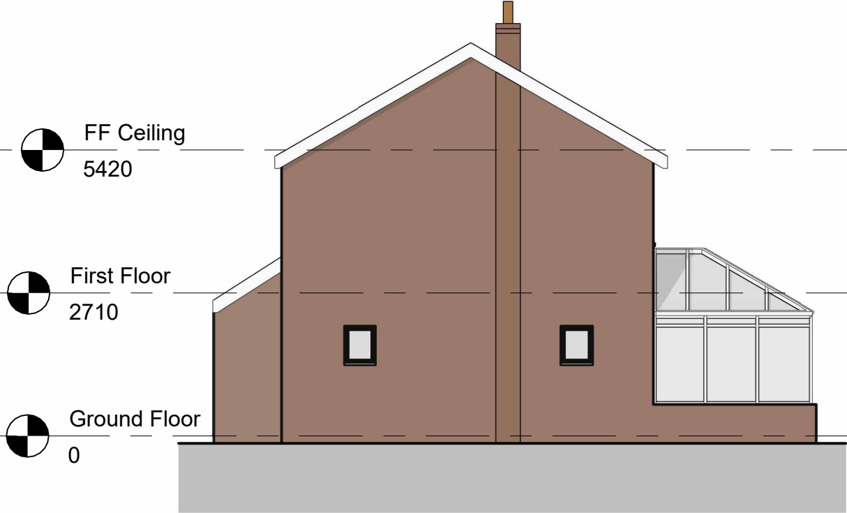
North West Elevation 1 : 100
