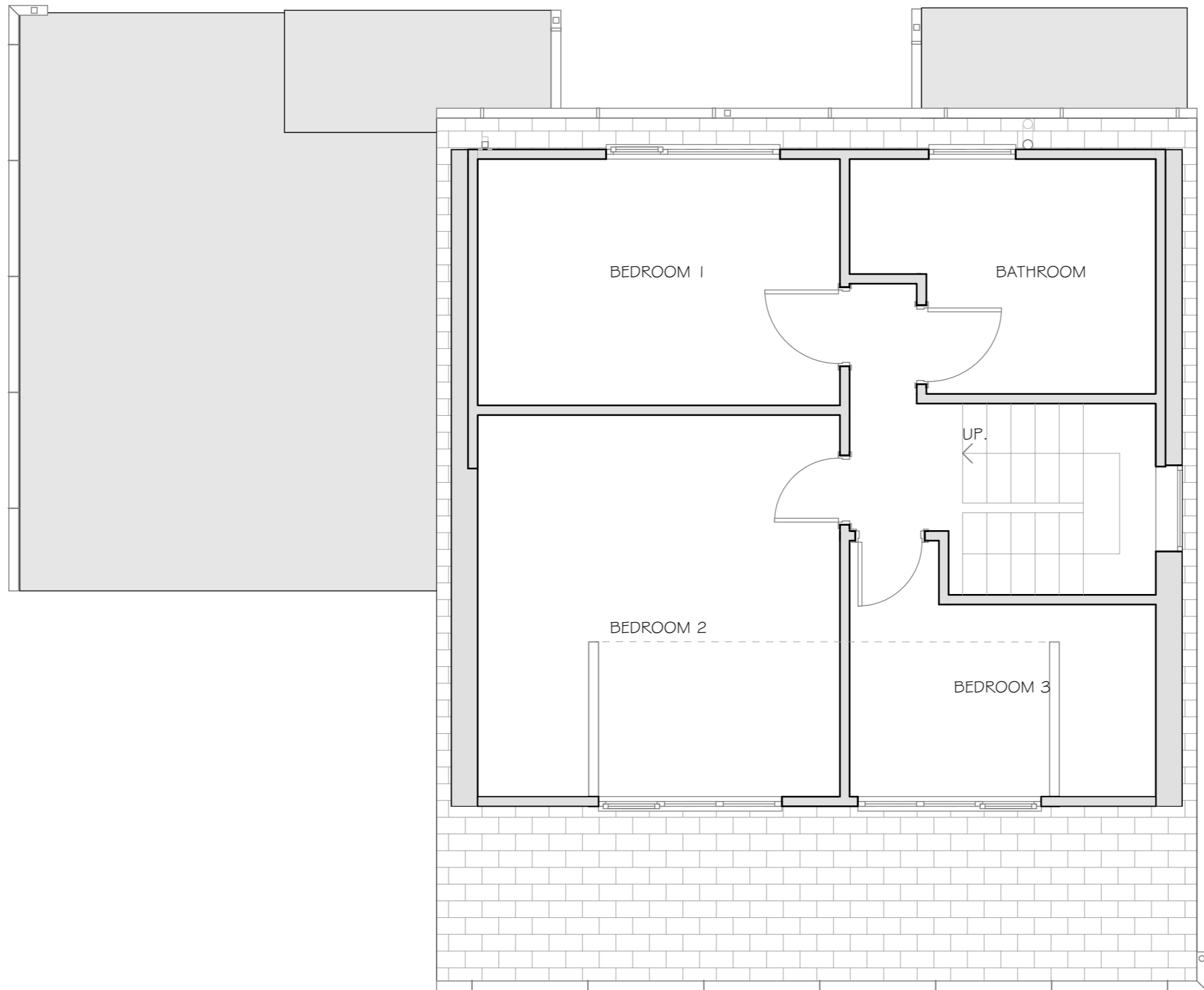
EXISTING FIRST FLOOR PLAN 1:50@A3
