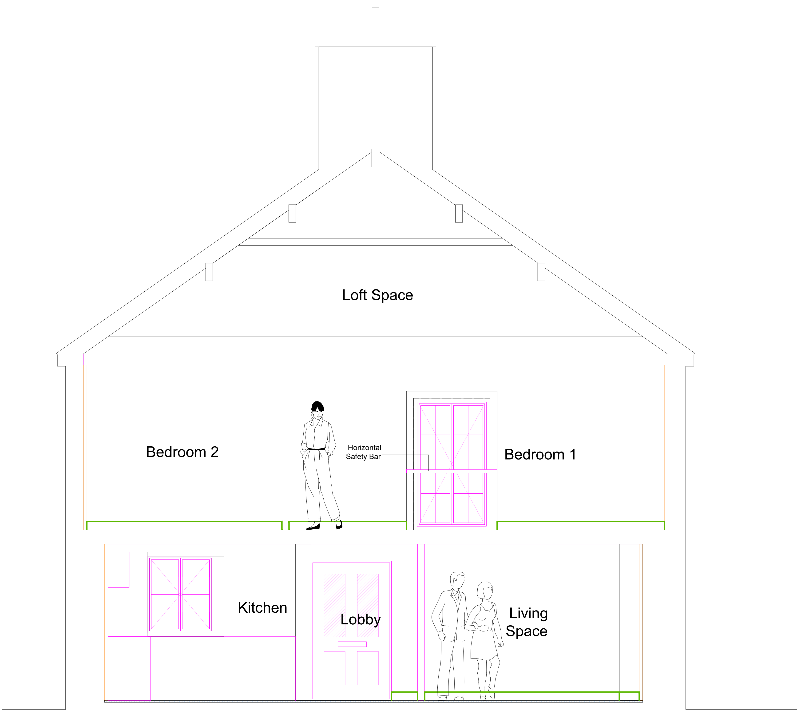
Section BB
