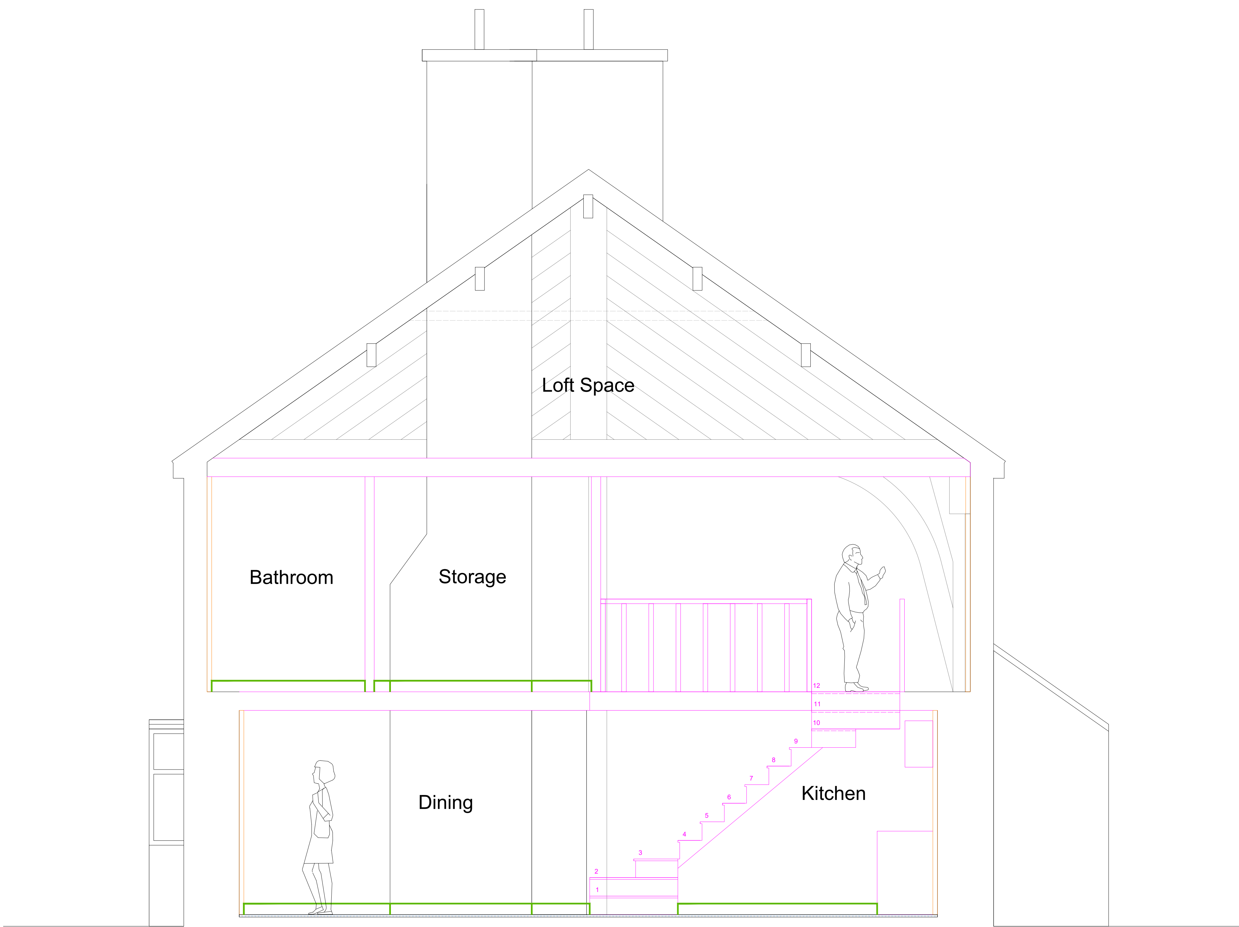
Section AA
