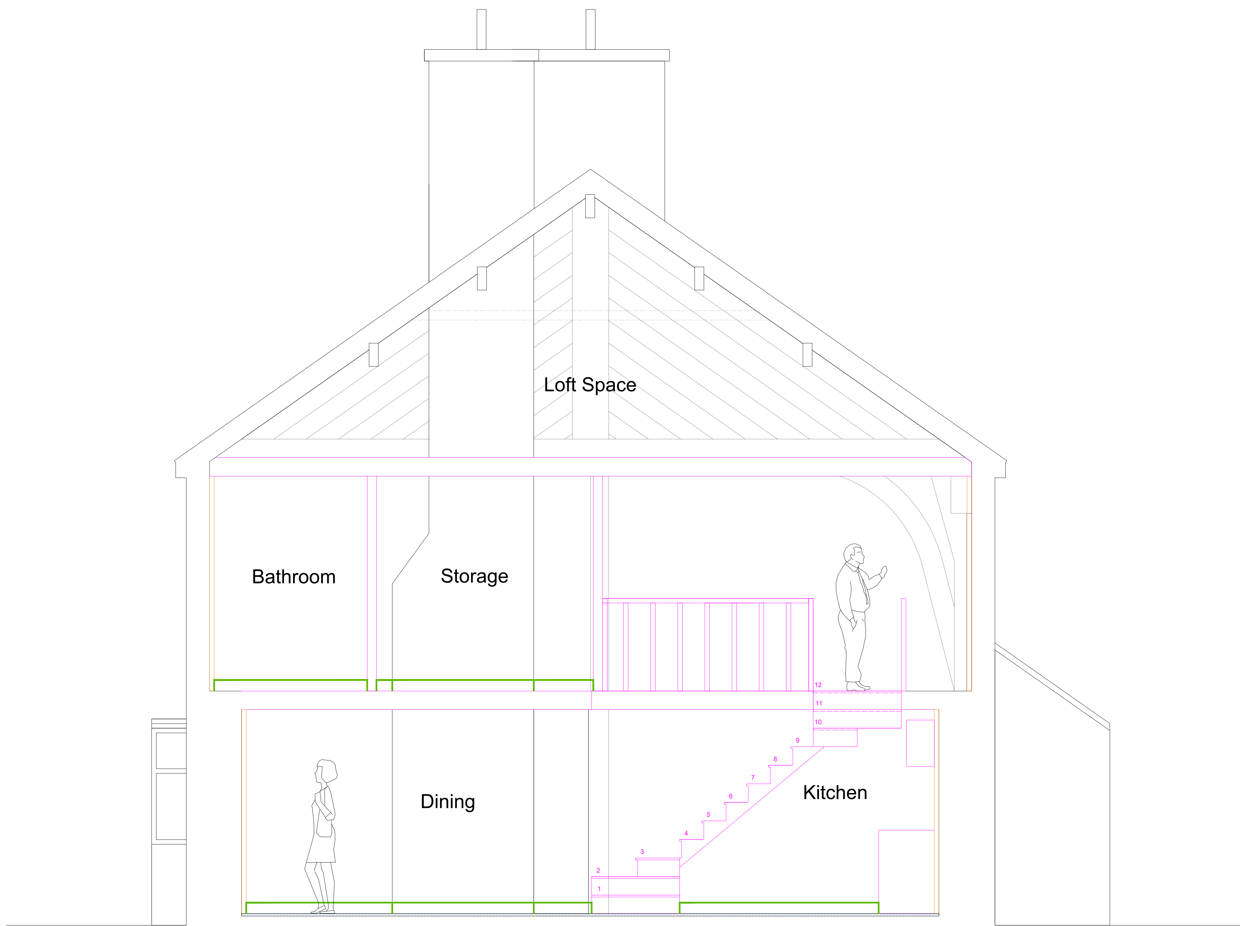
Section AA
