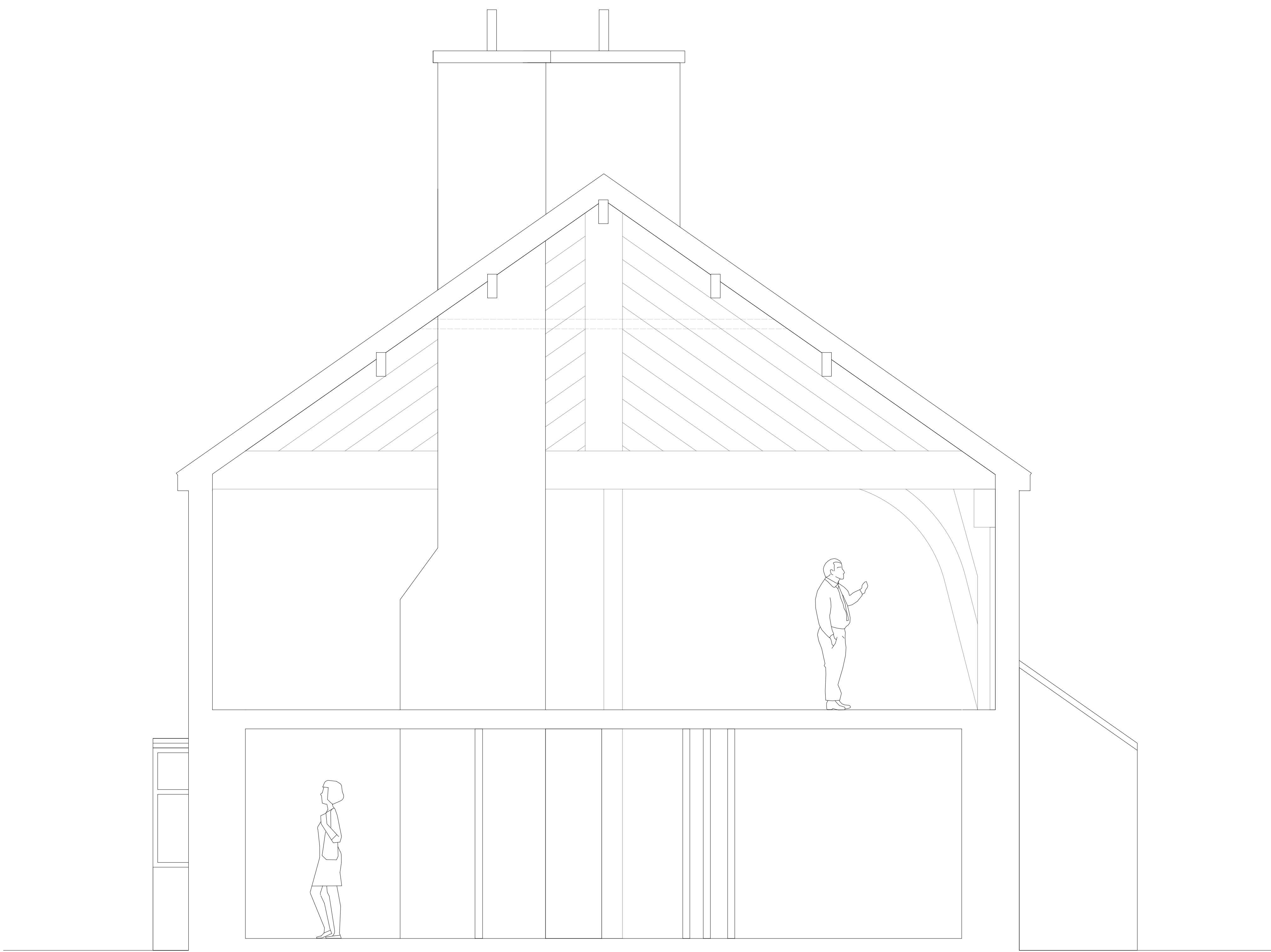
Section AA
