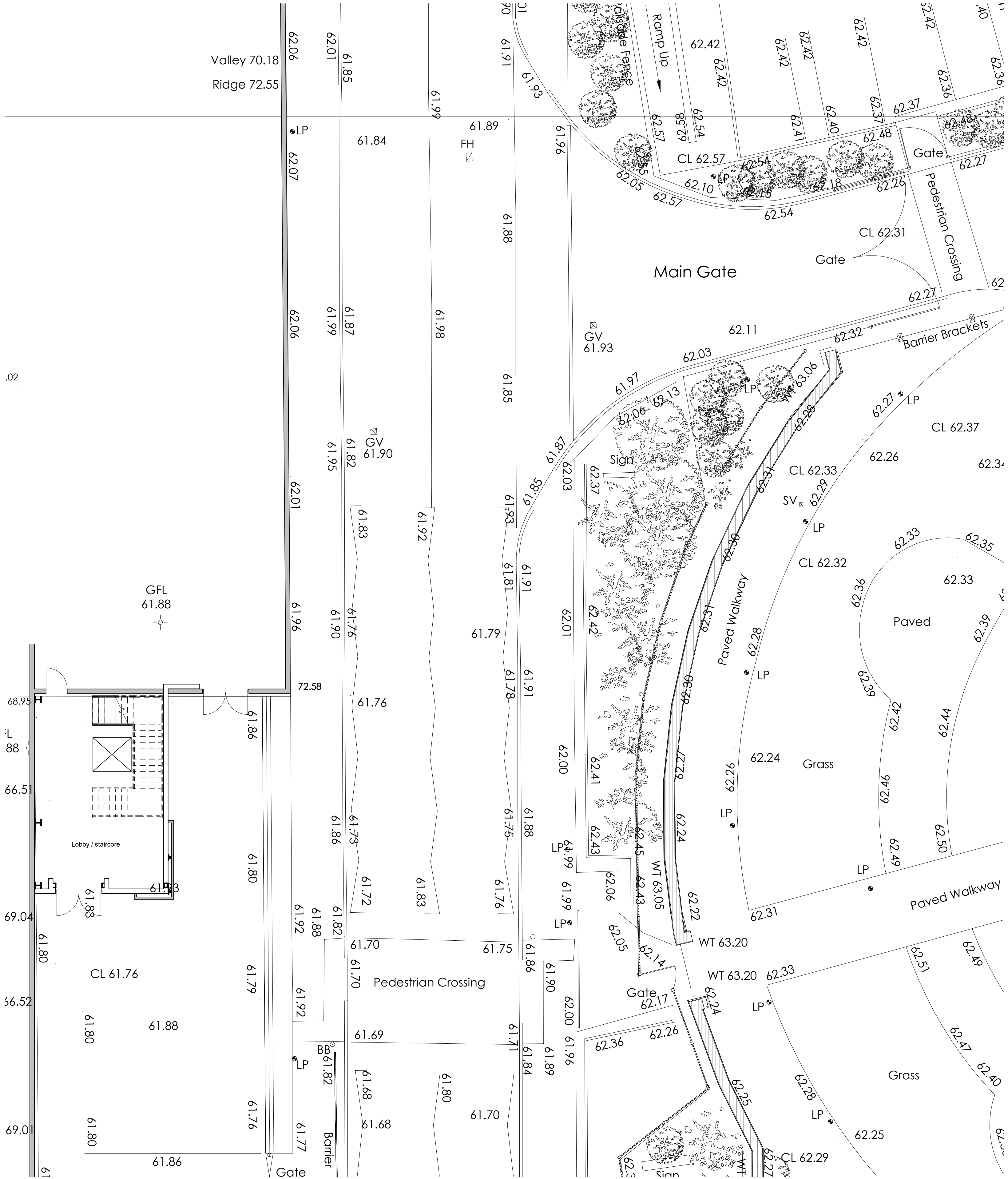
Ground Floor Existing 1 : 100
