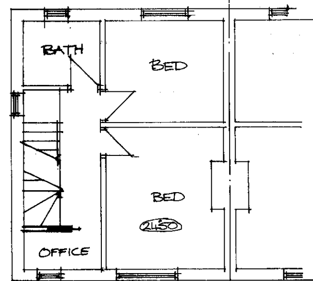
FIRST 1:100
