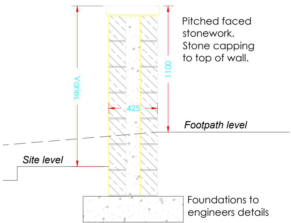
DETAIL A TYPICAL SECTION THROUGH BOUNDARY TREATMENT 01 SCALE 1:20
