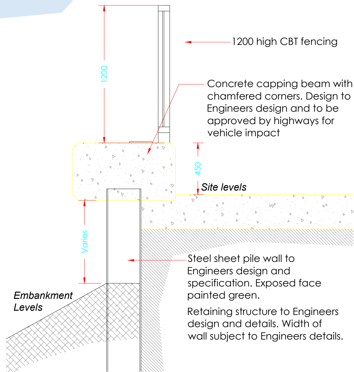
DETAIL B TYPICAL SECTION THROUGH BOUNDARY TREATMENT 03 SCALE 1:20
