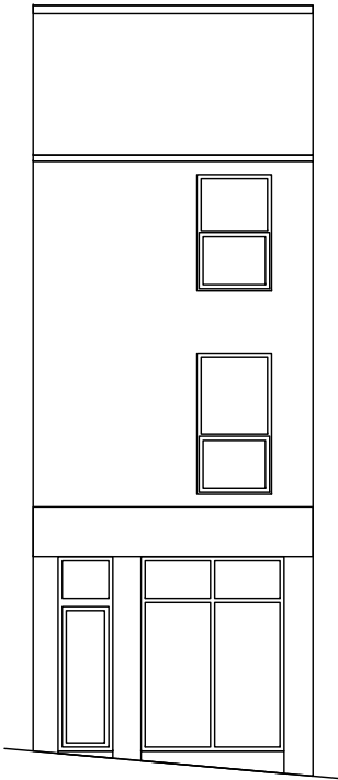
EXISTING FRONT ELEVATION
